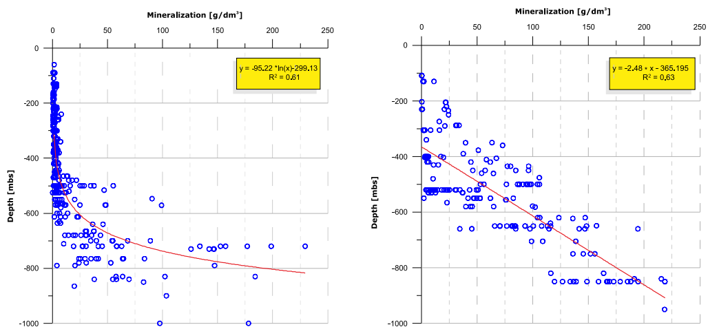
Fig. 4. Changes of groundwater mineralization with depth in the hydrogeological subregions of the USC B (after: A. Rózkowski ed., 2004)
