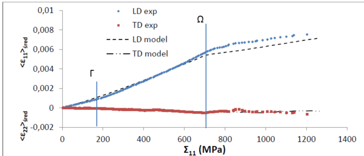
Fig. 2 Model and experimental relations \langle \epsilon_{11} \rangle and \langle \epsilon_{11} \rangle vs. \Sigma_{11} after initial stresses were taken into account – ferritic phase
