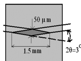
Fig. 5. Examined volume and its shape for synchrotron radiation
