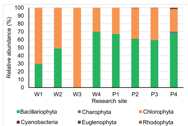
Fig. 11. Composition (%) of phytoplankton in Warna and Pengilon lakes; W = Lake Warna, P = Lake Pengilon; source: own study
