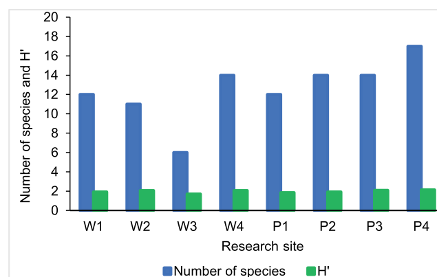
Fig. 12. The number of species and Shannon–Wiener diversity index ( H' ) in Pengilon and Warna lakes; W = Lake Warna, P = Lake Pengilon; source: own study
