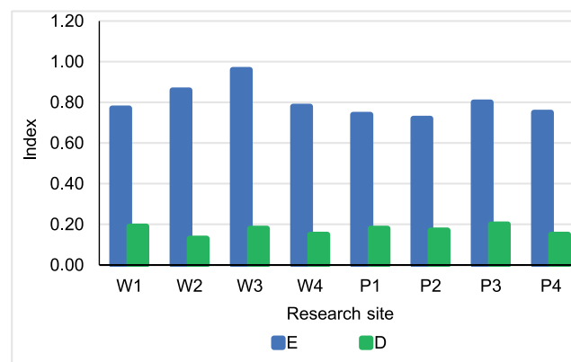
Fig. 13. The evenness index ( E ) and dominance index ( D ) in Pengilon and Warna Lakes, Dieng; W = Lake Warna, P = Lake Pengilon; source: own study
