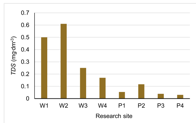
Fig. 7. Total dissolved solids (TDS) in Warna and Pengilon Lakes, April 2019; W = Warna Lake, P = Pengilon Lake; source: own study
