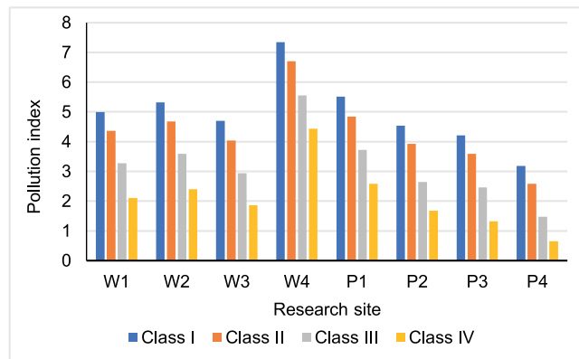
Fig. 10. Pollution index for water in Warna and Pengilon lakes, Dieng; W = Lake Warna, P = Lake Pengilon, class I = a source for drinking water, class II = for recreation, livestock and fish farming, class III = for livestock, fish farming, and agriculture, class IV = for agriculture; source: own study
