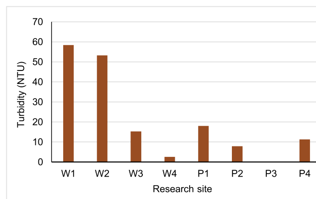
Fig. 6. Turbidity in Warna and Pengilon Lakes, April 2019; W = Warna Lake, P = Pengilon Lake; source: own study
