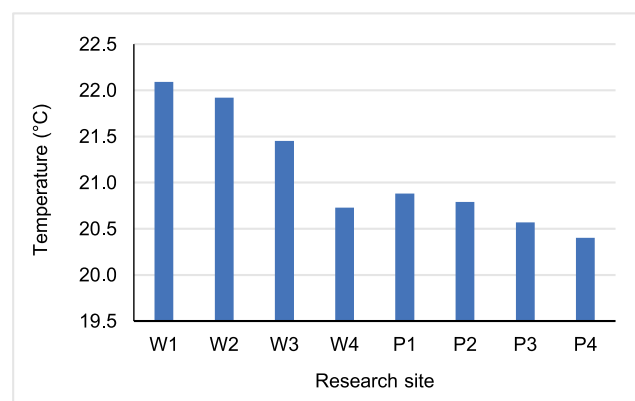
Fig. 3. Temperature of water in Warna and Pengilon lakes, April 2019; W = Lake Warna, P = Lake Pengilon; source: own study
