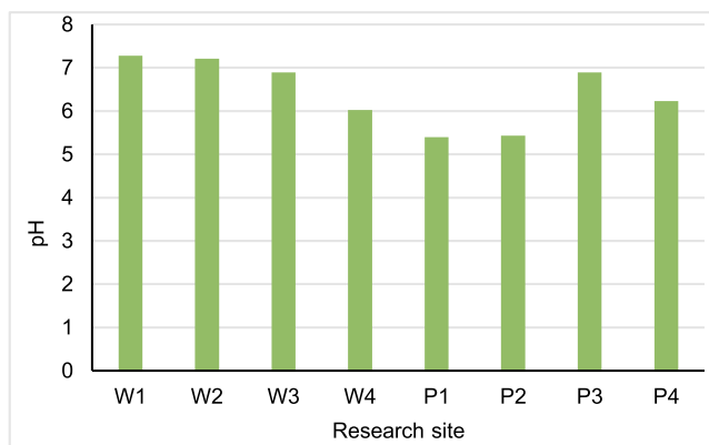
Fig. 5. pH of water in Warna and Pengilon Lakes, April 2019; W = Lake Warna, P = Lake Pengilon; source: own study
