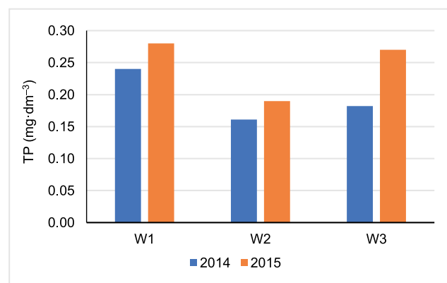
Fig. 9. Total phosphorus (TP) in water of Lake Warna, Dieng, 2014–2015; W1, W2, W3 = research sites; source: own elaboration based on SOEPROBOWATI et al. [2017]
