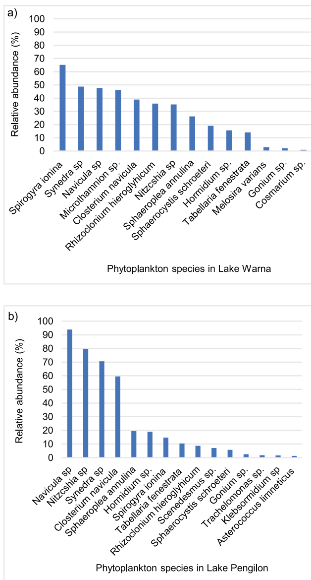
Fig. 14. The phytoplankton species with relative abundance >1% in investigated lakes: a) Lake Warna, b) Lake Pengilon; source: own study
