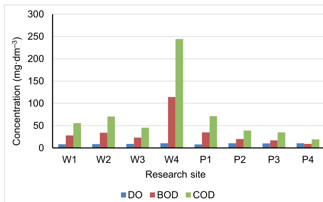
Fig. 4. Dissolved oxygen (DO), biological oxygen demand (BOD), and chemical oxygen demand (COD) in water of Warna and Pengilon lakes, April 2019; W = Lake Warna, P = Lake Pengilon; source: own study
