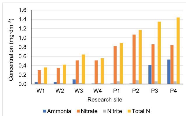
Fig. 8. Nitrogen compounds in water of Warna and Pengilon lakes, April 2019; W = Lake Warna, P = Lake Pengilon, total N = total nitrogen; source: own study
