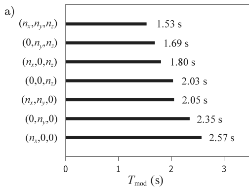
Fig. 10. a) Modal decay time T_{\text{mod}} for different types of modes, b) changes in the ratio M_{\text{mod}}/M with increasing the cutoff frequency f_c .
