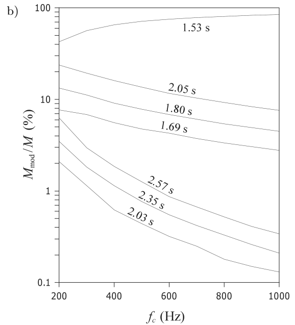
Fig. 10. a) Modal decay time T_{\text{mod}} for different types of modes, b) changes in the ratio M_{\text{mod}}/M with increasing the cutoff frequency f_c .
