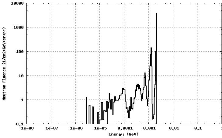
Fig. 2. Andreyivanovite neutron fluence for 252 Cf source
