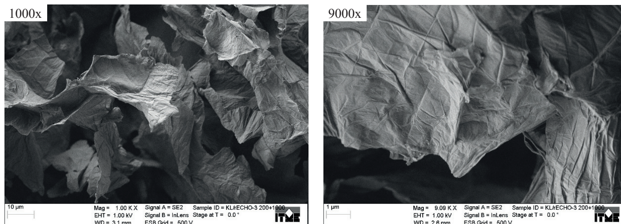
Fig. 1. SEM image of thermally reduced graphene oxide. Rys. 1. Obraz SEM rGO.
