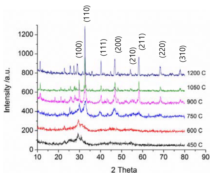
Fig. 1. XRD patterns of \text{Li}_{0.3}\text{La}_{0.57}\text{TiO}_3 annealed at different temperatures
