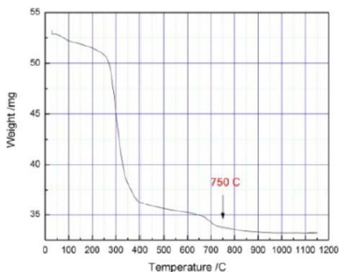
Fig. 2. TGA analysis of \text{Li}_{0.3}\text{La}_{0.57}\text{TiO}_3
