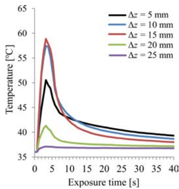
Fig. 4. Averaged for three tissue samples temperature rises induced in ex vivo pork loin tissue by the HIFU beam with an acoustic power of 24 W, pulse duration of 20 \mu s and duty-factor of 0.2. The maximum value of the standard deviation with increasing depth was \pm 5.5^\circ\text{C} , \pm 5.6^\circ\text{C} , \pm 7.3^\circ\text{C} , \pm 2.5^\circ\text{C} , \pm 0.7^\circ\text{C} , respectively.
