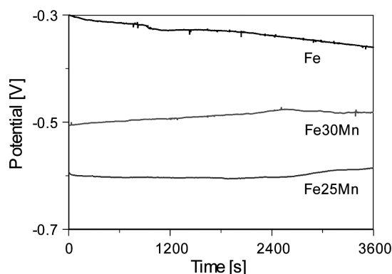
Fig. 3. The time evolution of the open-circuit potential of Fe, Fe-25wt.%Mn, Fe-30wt.%Mn electrodes immersed in Hank's solution
