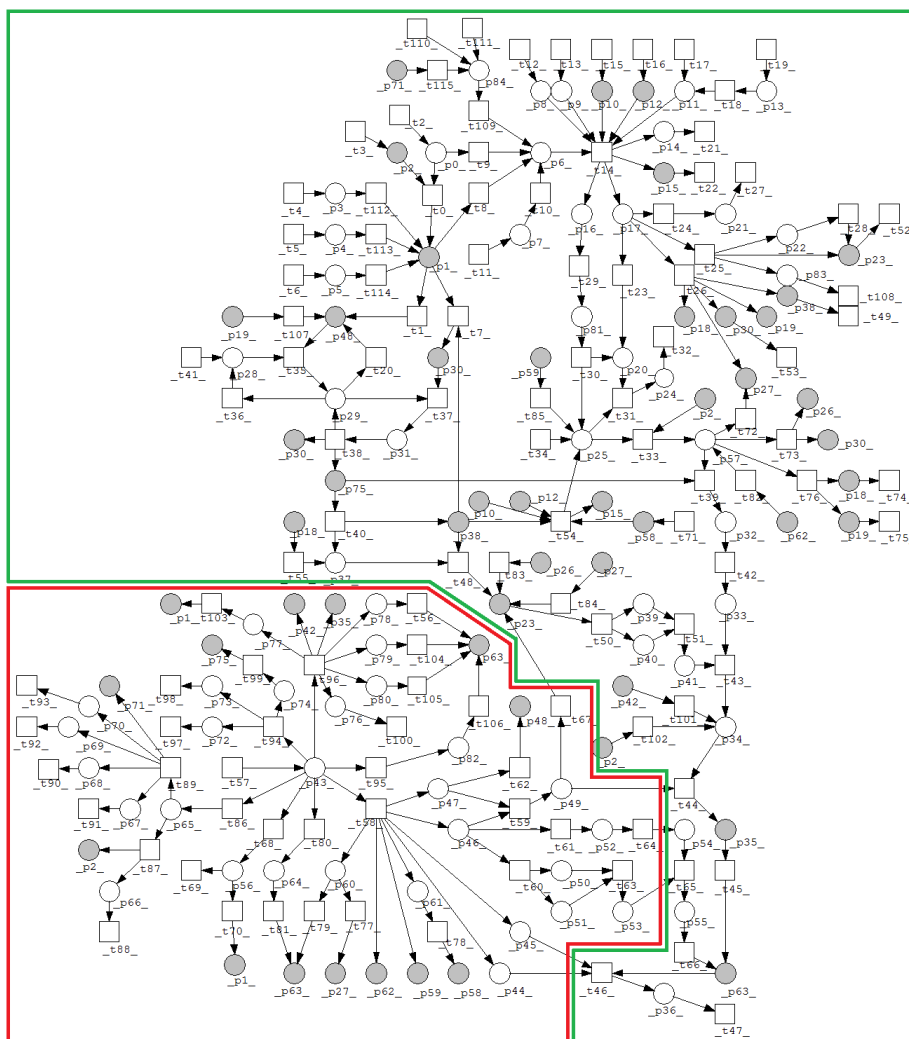
Figure 3: The proposed model is divided into two subnets: the upper frame presents mechanisms and molecules which are present in human organism and the lower frame presents mechanisms and harmful molecules which are associated with cigarette smoke.
