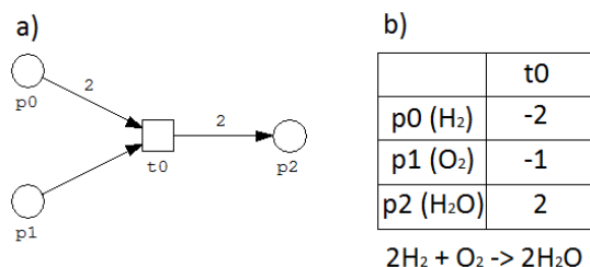
Figure 1: a) A graphical representation of a simple Petri net modeling synthesis of water; b) an incidence matrix of the net presented in part a).
