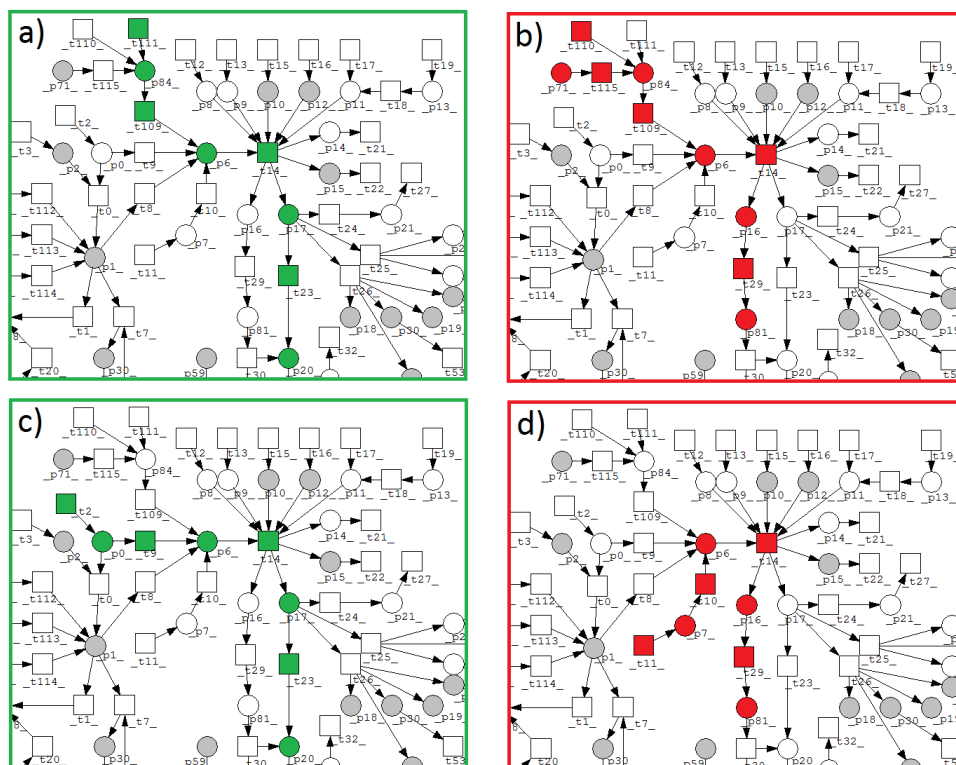
Figure 4: Simplifications caused by inhibition reactions: the left frames a) and c) correspond to situations in normal conditions and the right frames b) and d) correspond to inhibition reactions.
