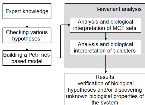
Figure 2: A scheme of work: through expert knowledge and checking various hypotheses to modeling and analysis of biological processes using Petri nets.
