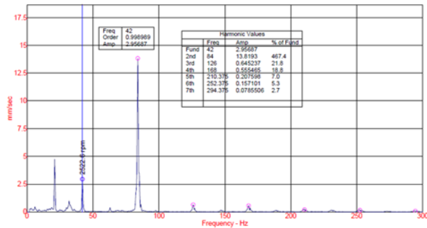
Fig 6. Typical vibration spectrum of a four stroke Otto engine
