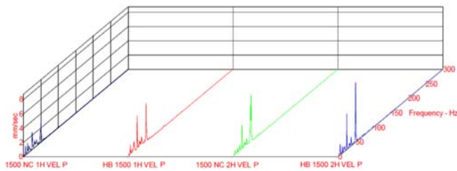
Fig 7. Effect of exhaust clogging on vibration spectrum
