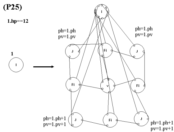
Fig. 22. Graph grammar production for breaking the interior of a rectangular element.
