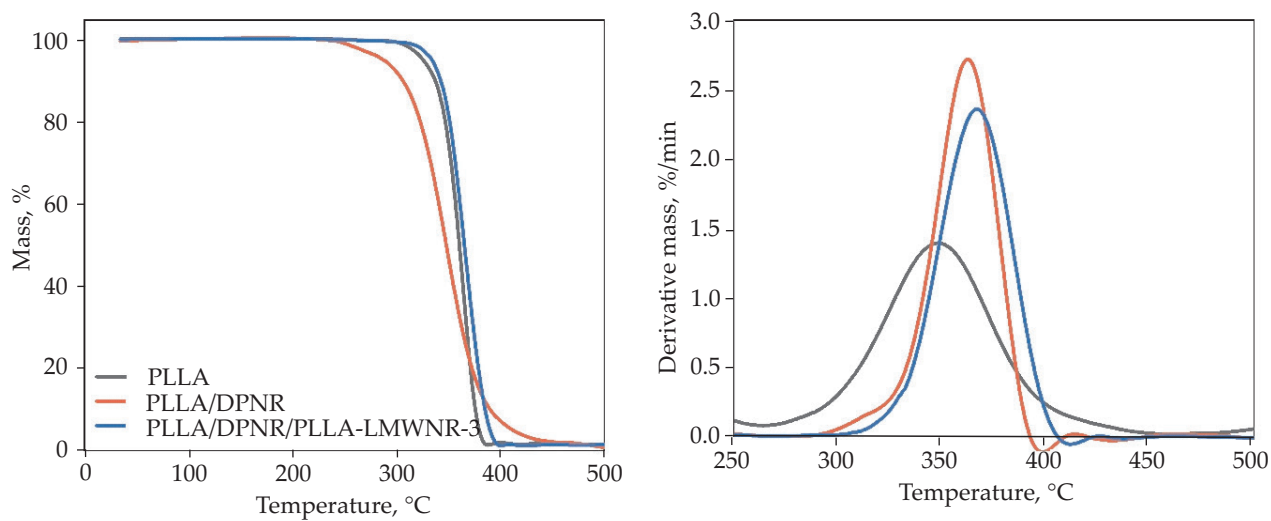
Fig. 5. TGA and DTG curves of PLLA blends
