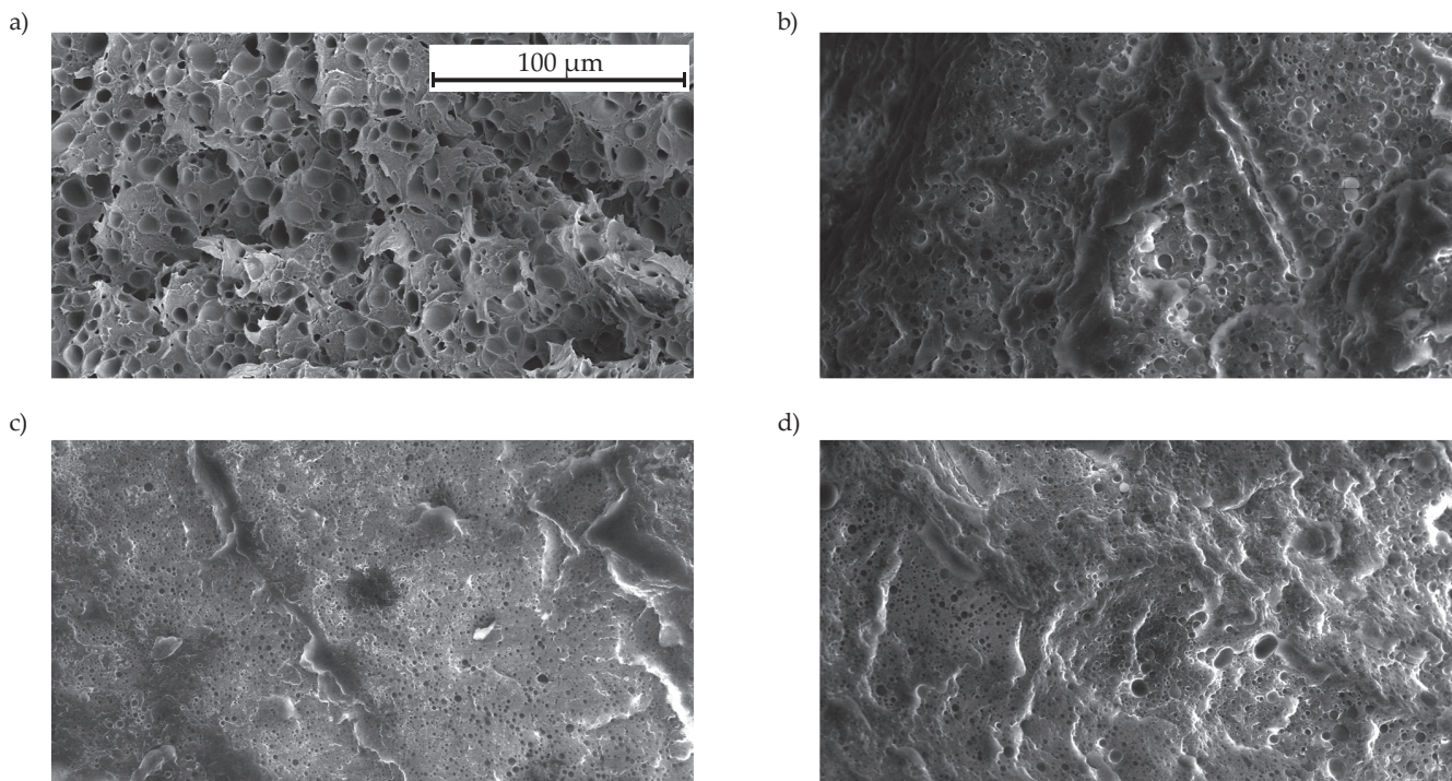
Fig. 4. Fracture surface morphology of: a) PLLA/DPNR, b) 3% PLLA/DPNR/PLLA-LMWNR-1, c) 3% PLLA/DPNR/PLLA-LMWNR-3, d) 3% PLLA/DPNR/PLLA-LMWNR-12
