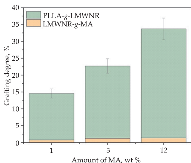
Fig. 2. Grafting degree of LMWNR-MA and PLLA-LMWNR
