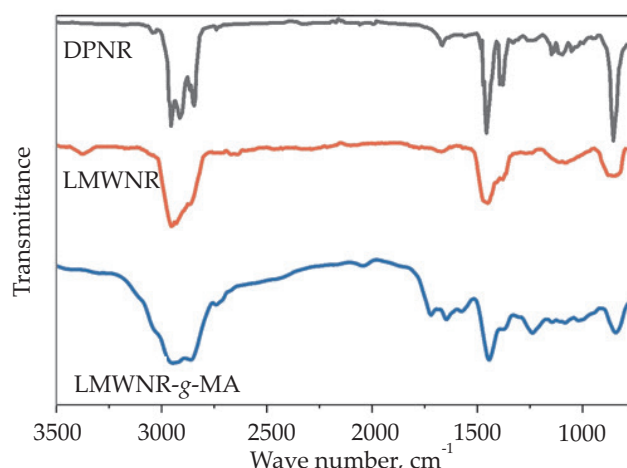
Fig. 1. FT-IR spectra of DPNR and modified DPNR
