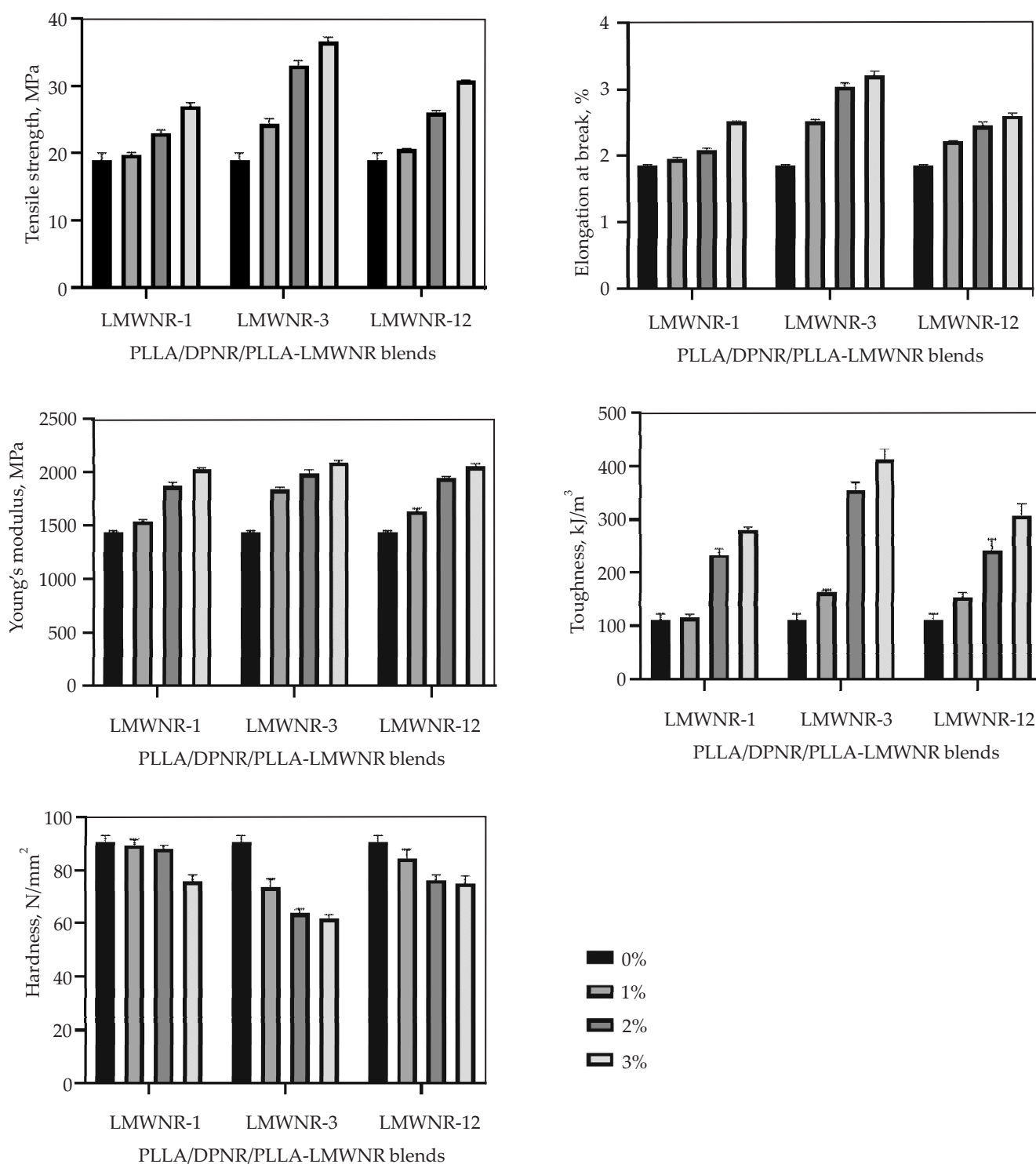
Fig. 3. Mechanical properties of PLLA/DPNR blends
