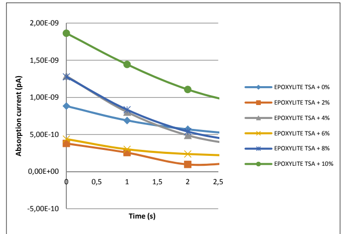
Fig. 10. Absorption currents on samples filled with Al 2 O 3
