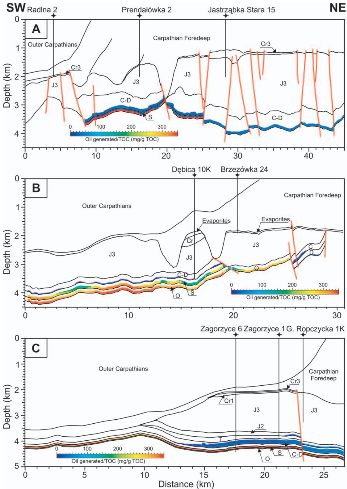
Fig. 2. Amount of generated oil along the A , B and C cross-sections. Cr – Cretaceous, Cr3 – Upper Cretaceous, Cr1 – Lower Cretaceous, J3 – Upper Jurassic, J2 – Middle Jurassic, T – Triassic, C – Carboniferous, D – Devonian, S – Silurian, O – Ordovician. Some of the wells were projected onto cross-sections. See Fig. 1 for location
