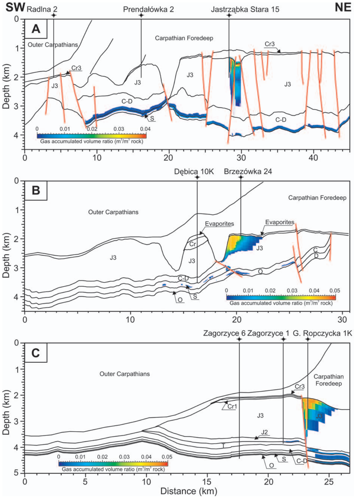
Fig. 6. The volume of the gas accumulation along the A, B and C cross-sections. See Fig. 1 for location and Fig. 2 for abbreviations
