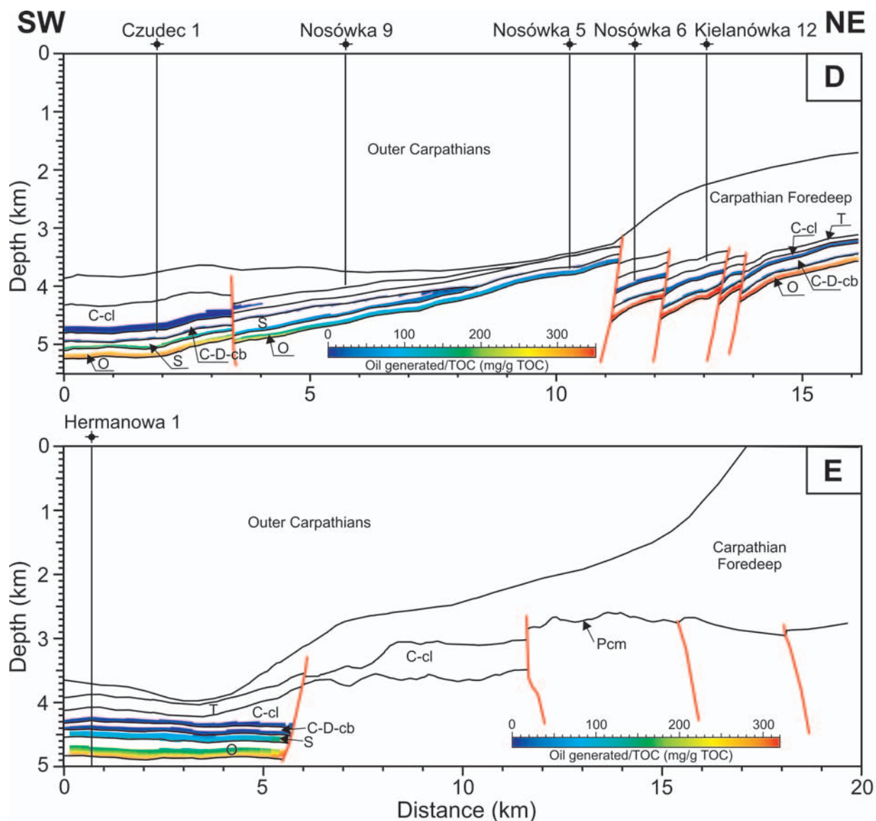
Fig. 7. Amount of generated oil along the D and E cross-sections. T – Triassic, C-cl – clastic strata of the Carboniferous, C-D-cb – carbonate strata of the Devonian and Carboniferous, S – Silurian, O – Ordovician, Pcm – Precambrian. Some of the wells were projected onto cross-sections. See Fig. 1 for location
