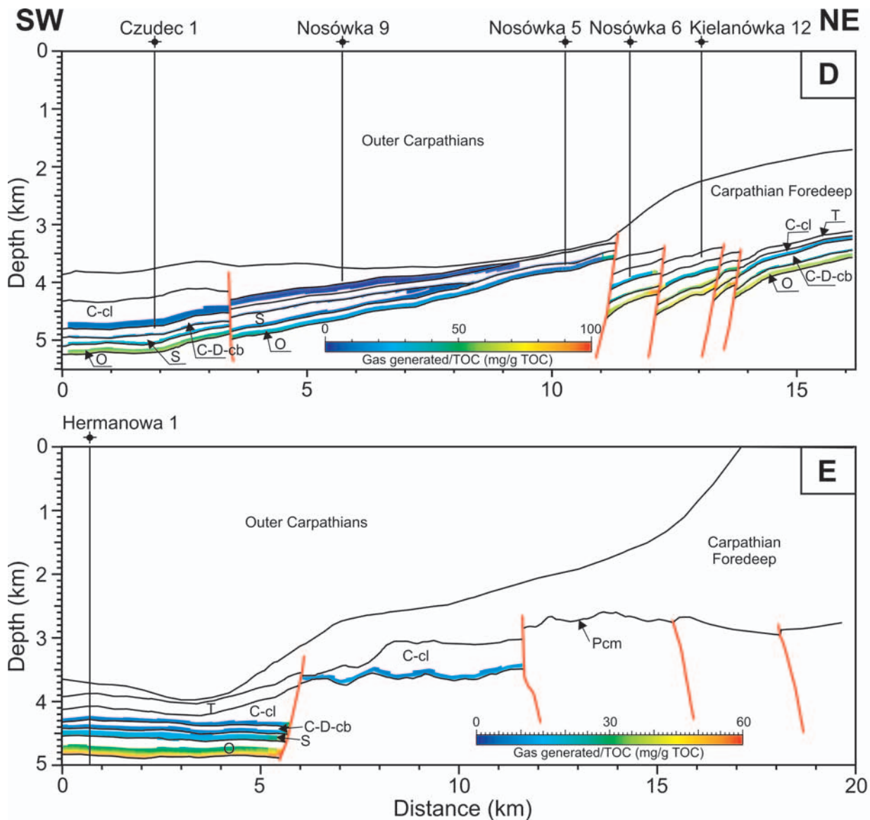
Fig. 8. Amount of generated gas along the D and E cross-sections. See Fig. 1 for location and Fig. 7 for abbreviations
