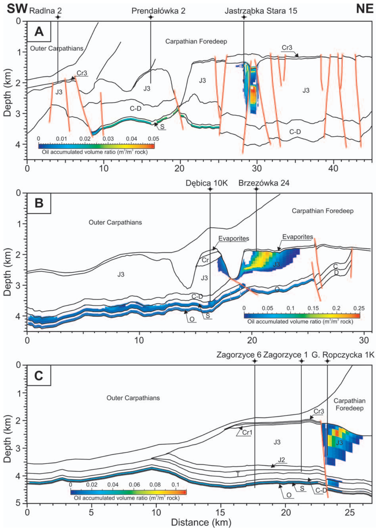
Fig. 5. The volume of the oil accumulation along the A, B and C cross-sections. See Fig. 1 for location and Fig. 2 for abbreviations
