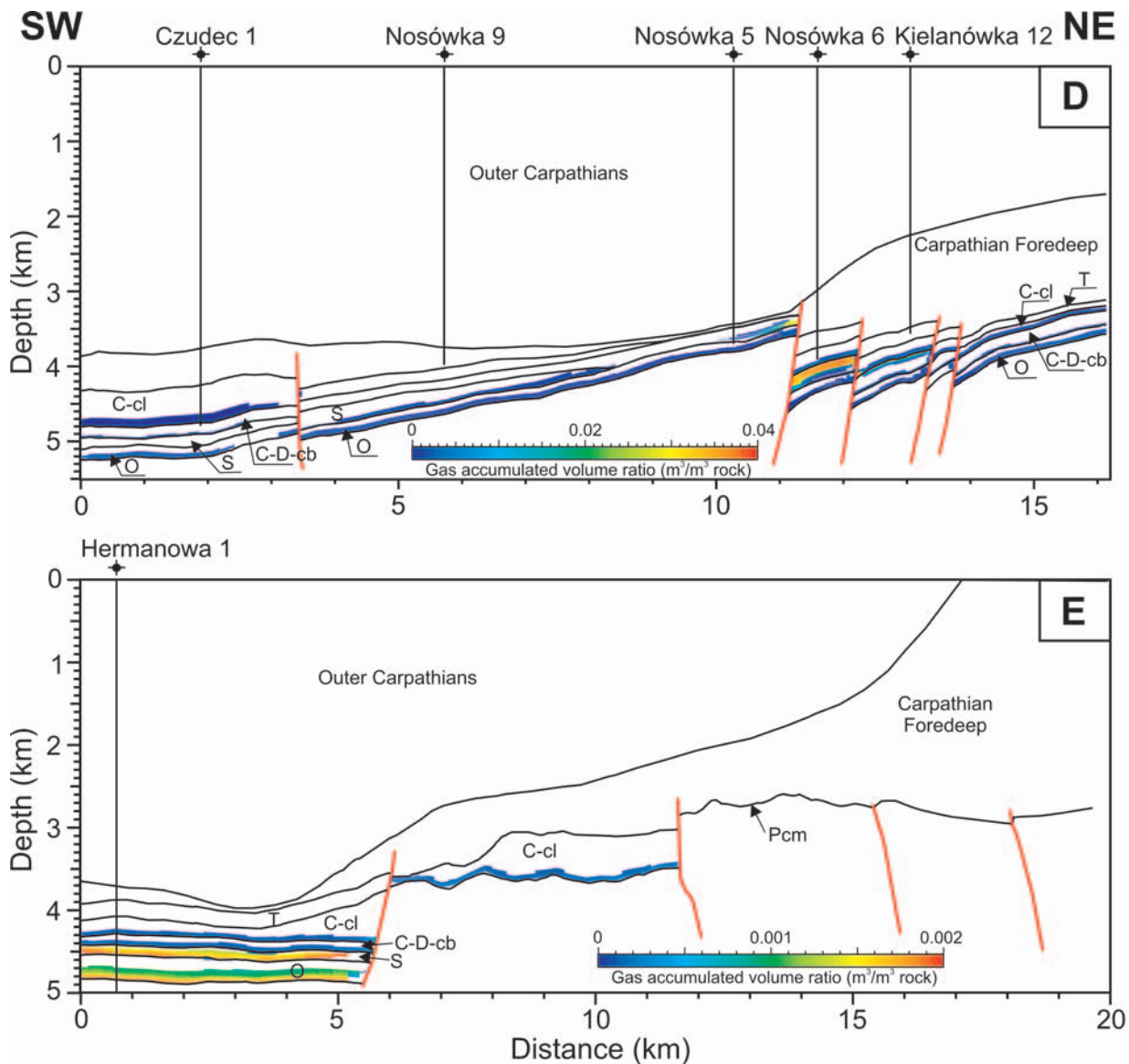
Fig. 10. The volume of the gas accumulation along the D and E cross-sections. See Fig. 1 for location and Fig. 7 for abbreviations
