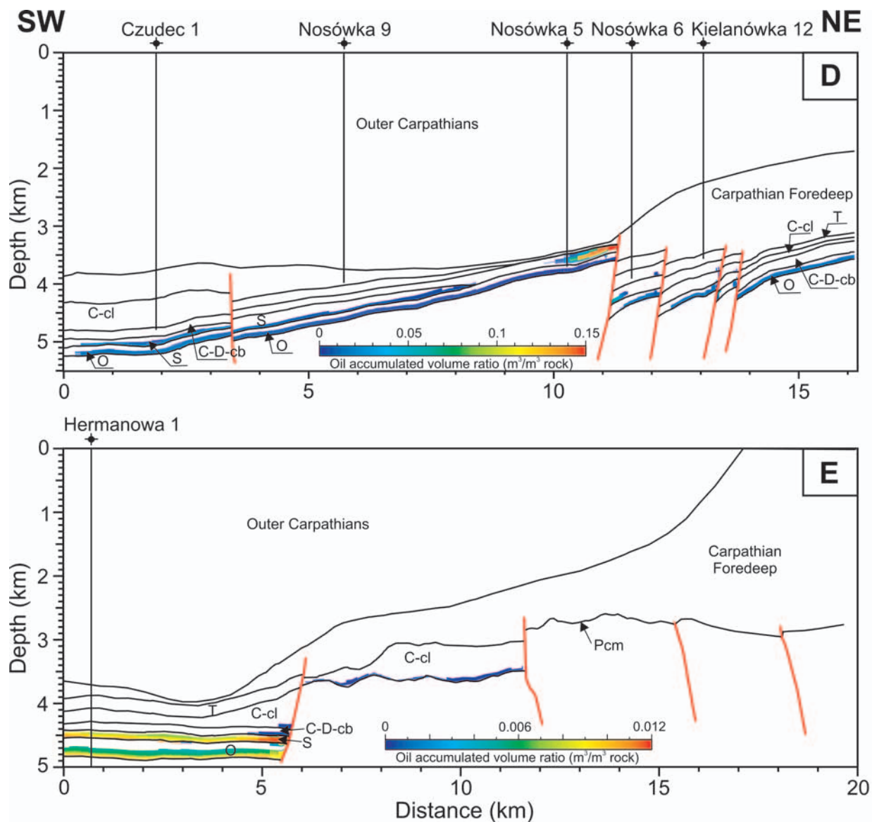
Fig. 9. The volume of the oil accumulation along the D and E cross-sections. See Fig. 1 for location and Fig. 7 for abbreviations
