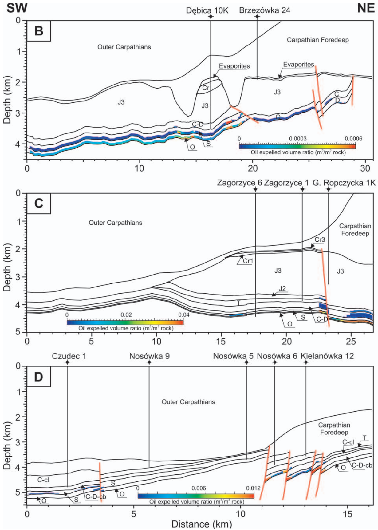
Fig. 4. The volume of the oil expulsion along the B, C and D cross-sections. See Fig. 1 for location and Figs 2 and 7 for abbreviations
