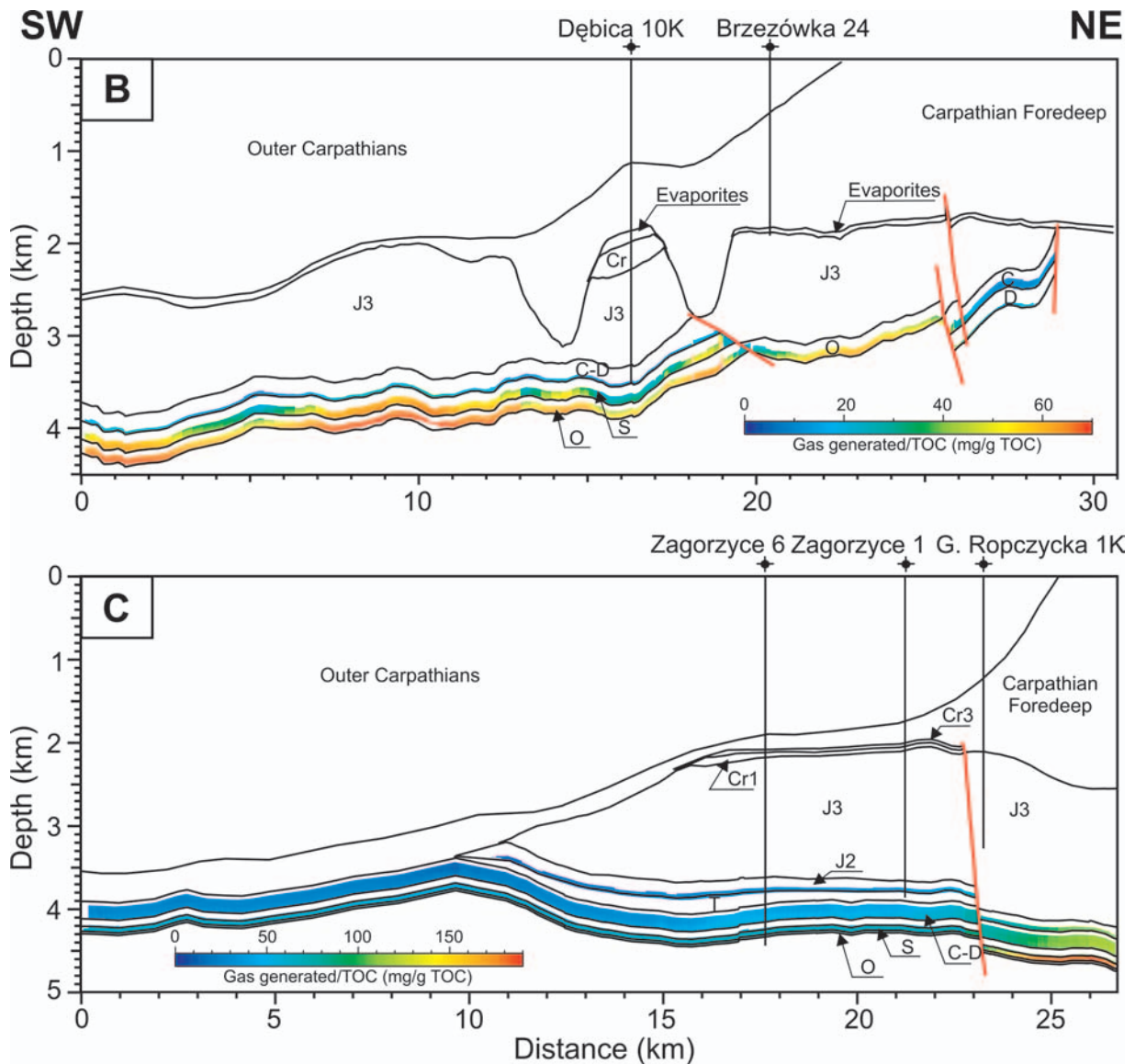
Fig. 3. Amount of generated gas along the B and C cross-sections. For abbreviations see Fig. 2
