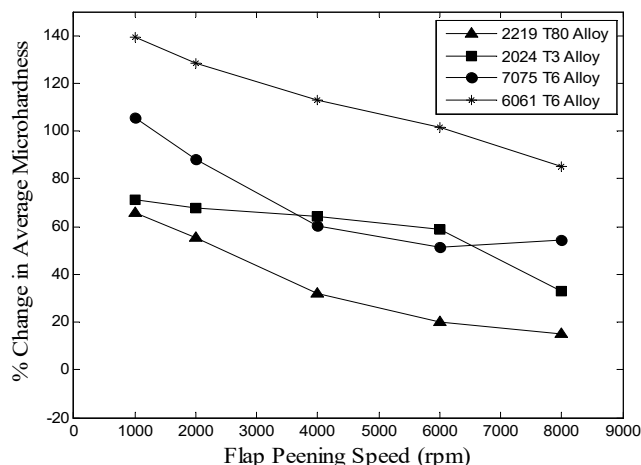
Fig. 4. The % change in average microhardness (HV) after flap peening for aluminum alloys
