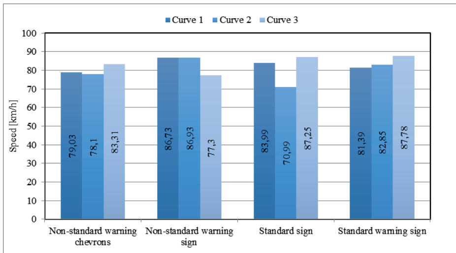
Fig. 5. Comparison of mean curve speed for different scenarios
