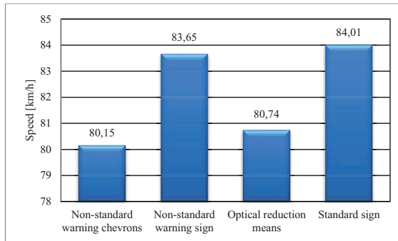
Fig. 6. Comparison of mean speeds within different experimental scenarios
