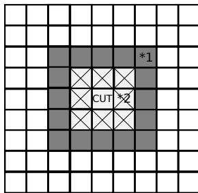
Fig. 6. The schema of the two dimensional CACFAR window. CUT - cell under test, *1 - window cells, *2 - guard cells
