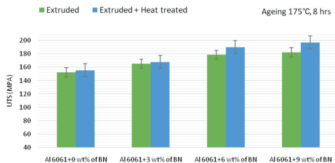
Fig. 4. Variation of UTS of hot extruded and heat-treated Al6061-BN composites
