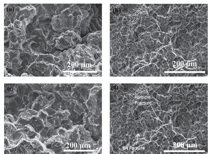
Fig. 8. The microstructure of fractured surface of extruded: a) Al6061 + 6 wt% of BN and (c) Al6061 + 9 wt% of BN. extruded + heat treated: (b) Al6061 + 6 wt% of BN and (d) Al6061 + 9 wt% of BN
