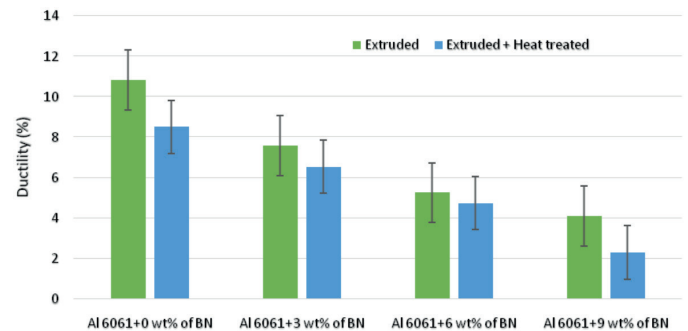
Fig. 7. Variation in ductility of hot extruded and extruded with heat-treated Al6061-BN composites
