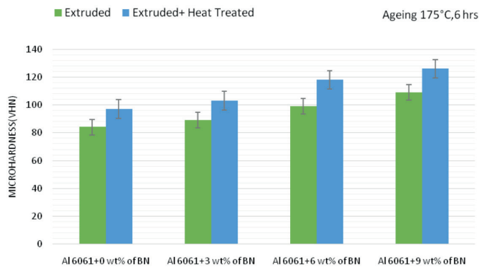
Fig. 2. Variation of micro-hardness of hot extruded and heat treated Al6061-BN composites with wt% of reinforcement
