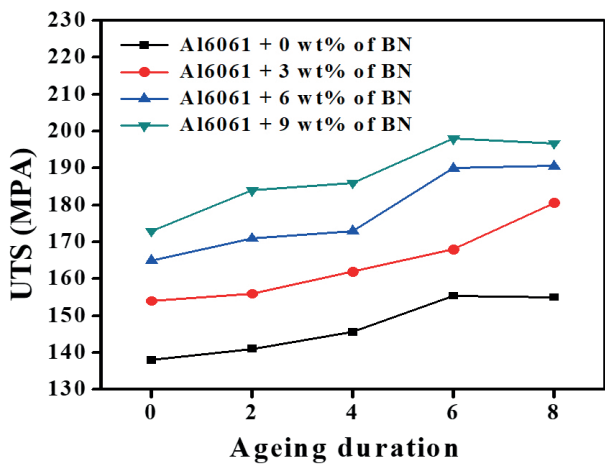
Fig. 5. Ageing duration effect on tensile-strength of Al6061-BN composites
