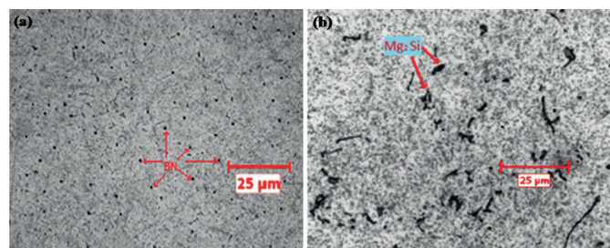
Fig. 1. Optical microphotographs of (a) extruded and (b) extruded + heat treatment specimens
