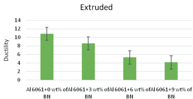
Fig. 6. Ductility variations of hot extruded Al6061 alloy and Al6061-BN composites
