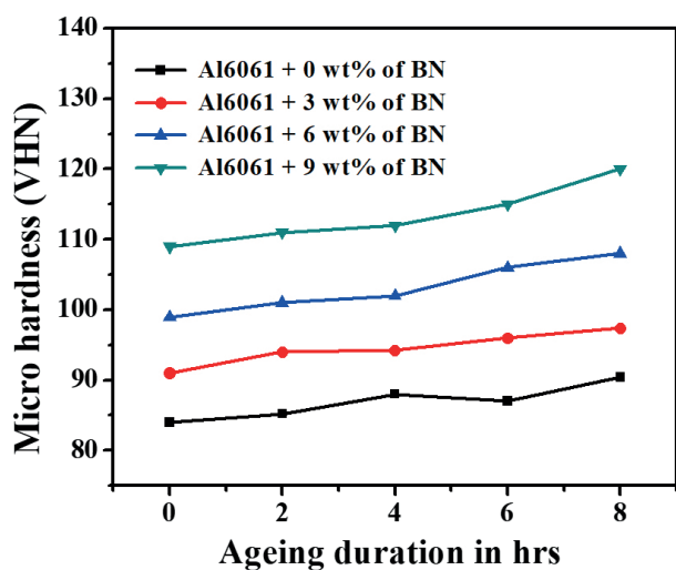
Fig. 3. Effect of ageing duration over micro harness of Al6061-BN composites
