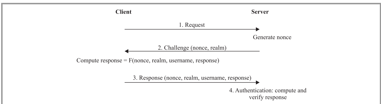
Fig. 2. SIP authentication.
