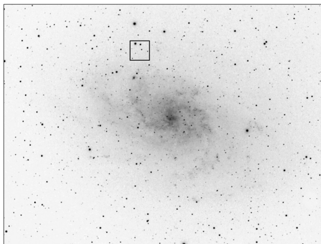
Fig. 1. A picture of M33 Galaxy, a group of stars is marked and chosen for the next calculation. The picture: Robert Suszyński, refractor SW80ED 80/600mm, camera SBIG ST-2000XM, stacking 13 images with exposure of 300 s each.
