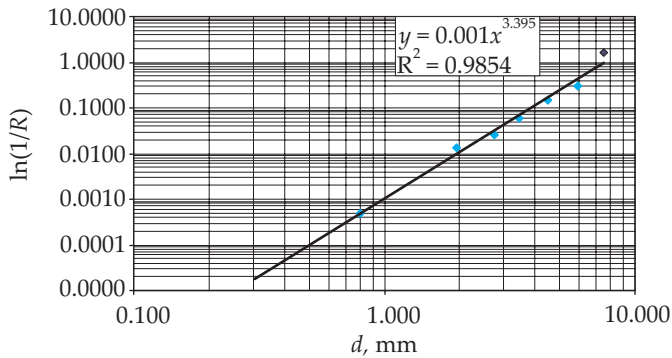
Fig. 7. Compliance of experimental points of particle size distribution for PP – \phi 10 mm with RRSB equation
