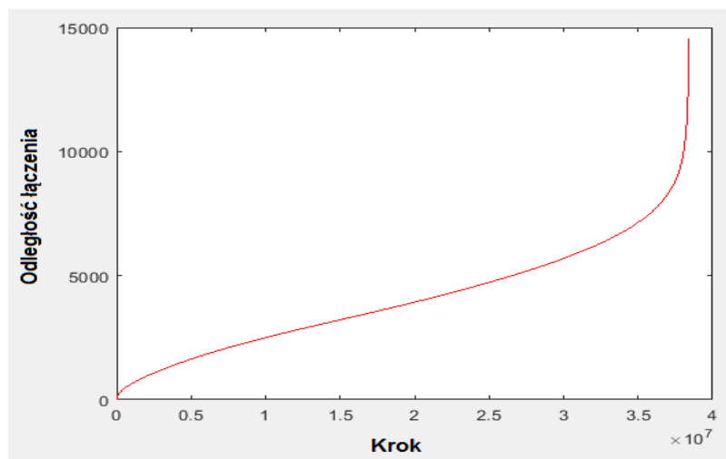
Figure 14. The course of the results of the agglomeration method for Ward's algorithm based on data on the work of JKSE in 2018. Descriptions: Krok (Pol.) – Step (Eng.), Odległość łączenia (Pol.) - Connecting distance. Source: Own elaboration using the Neural Network Toolbox of MATLAB and Simulink [5-6, 18, 20, 28].
