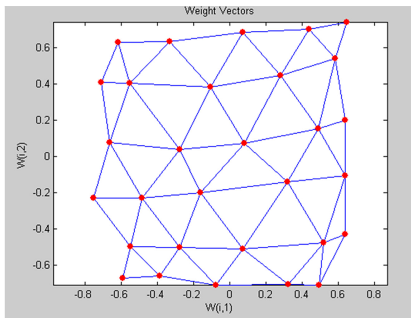
Figure 2. Graph visualizing the last step in creating a neuron mesh Markings: W(i, 1) - weight of the X axis, W(i, 2) - weight of the Y axis, Source: Own elaboration in MATLAB and Simulink environment [6, 18, 31].
