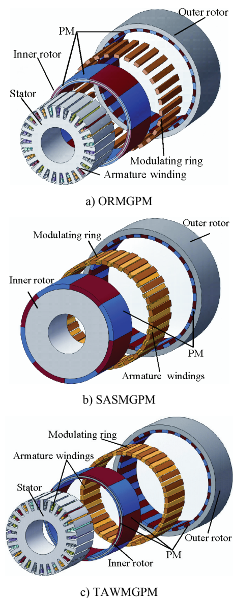
Fig. 2. Topology structure of MGPM electrical machine
