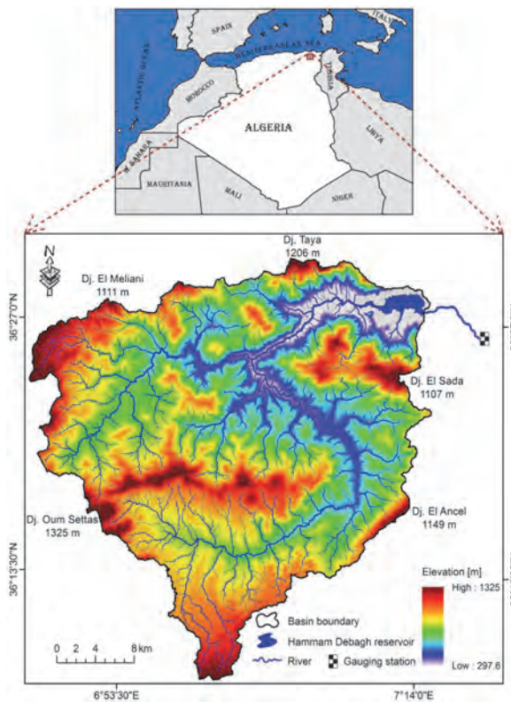
Fig. 1. Localization of the study area; source: own elaboration
