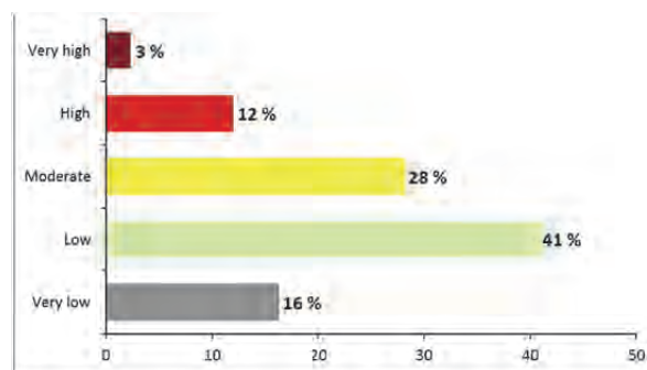
Fig. 14. Distribution of erosion risk classes in the Bouhamdane watershed; source: own study
