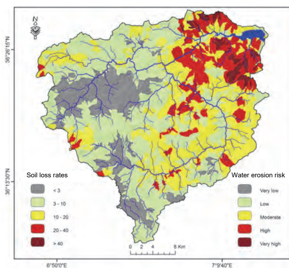
Fig. 13. Soil loss rates ( t \cdot ha^{-1} \cdot y^{-1} ) and erosion risk map in the Bouhamdane watershed; source: own study
