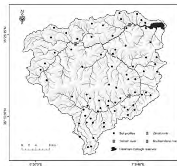
Fig. 4. Distribution of soil profiles analyzed in the Bouhamdane watershed; source: own elaboration based on the National of Forestry Studies' data
