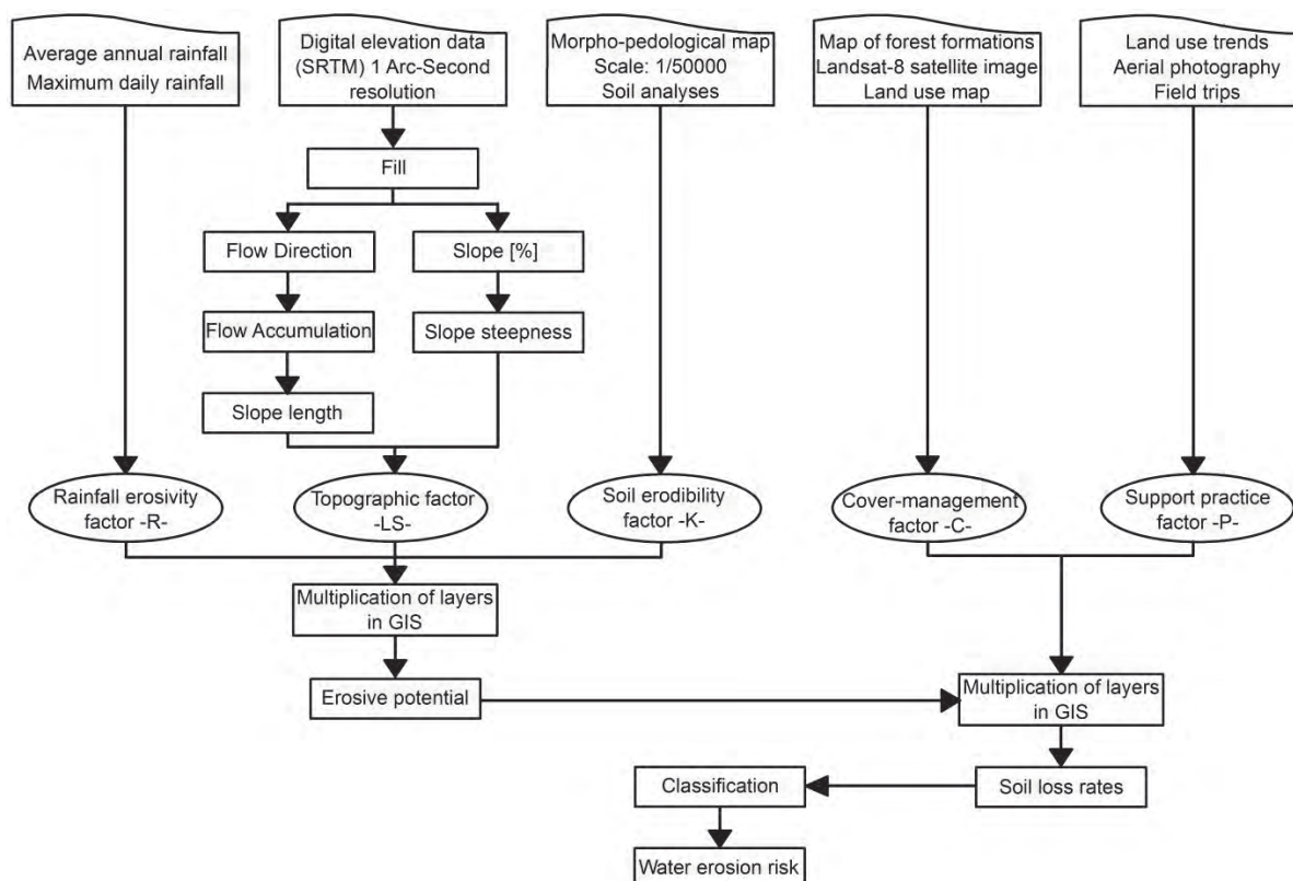
Fig. 2. Chart of the adopted methodology; source: own elaboration
