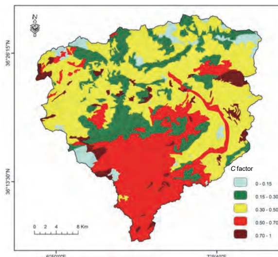
Fig. 10. C factor distribution map in the Bouhamdane watershed; source: own study
