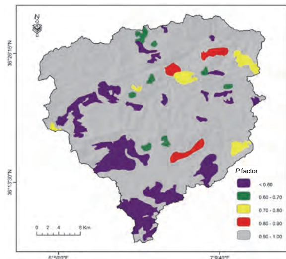
Fig. 12. P factor distribution map in the Bouhamdane watershed; source: own study
