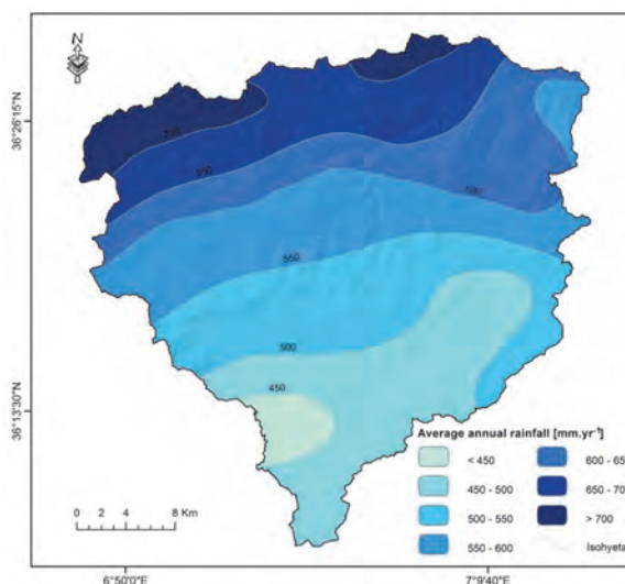
Fig. 3. Map of average annual precipitation in the Bouhamdane watershed; source: own elaboration
