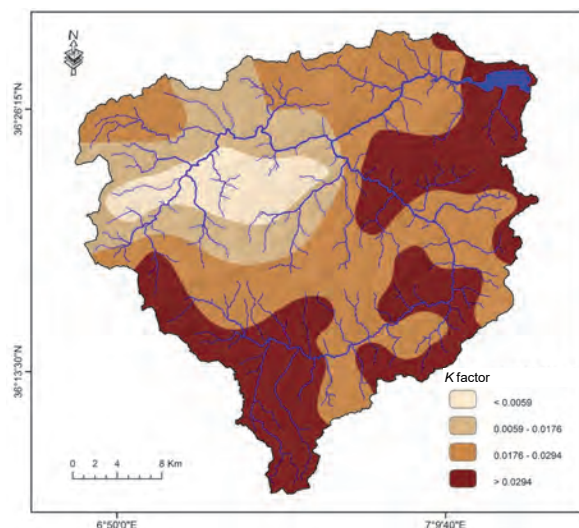
Fig. 9. K factor ( t \cdot ha \cdot h \cdot ha^{-1} \cdot MJ^{-1} \cdot mm^{-1} ) distribution map in the Bouhamdane watershed; source: own study
