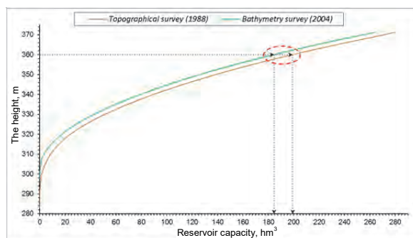
Fig. 15. Height-capacity curves of Hammam Debagh Dam; source: own study
