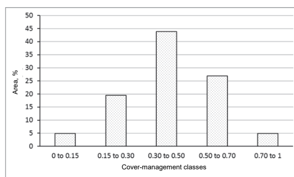
Fig. 11. Distribution of cover-management classes; source: own study
