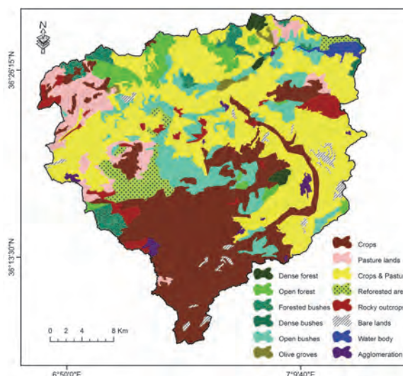
Fig. 5. Land-use map of the Bouhamdane watershed; source: own elaboration
