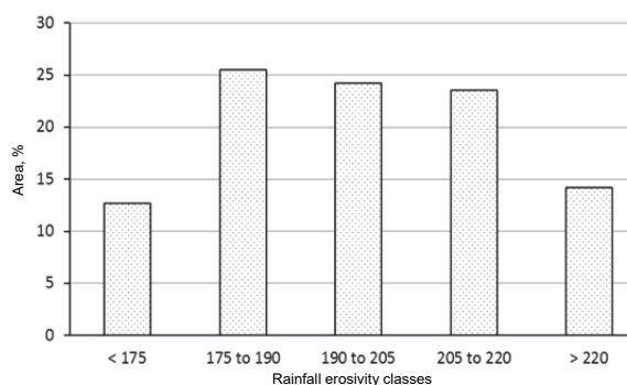
Fig. 7. Distribution of rainfall erosivity classes; source: own study
