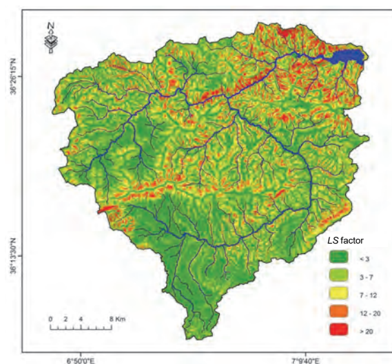
Fig. 8. LS factor distribution map in the Bouhamdane watershed; source: own study
