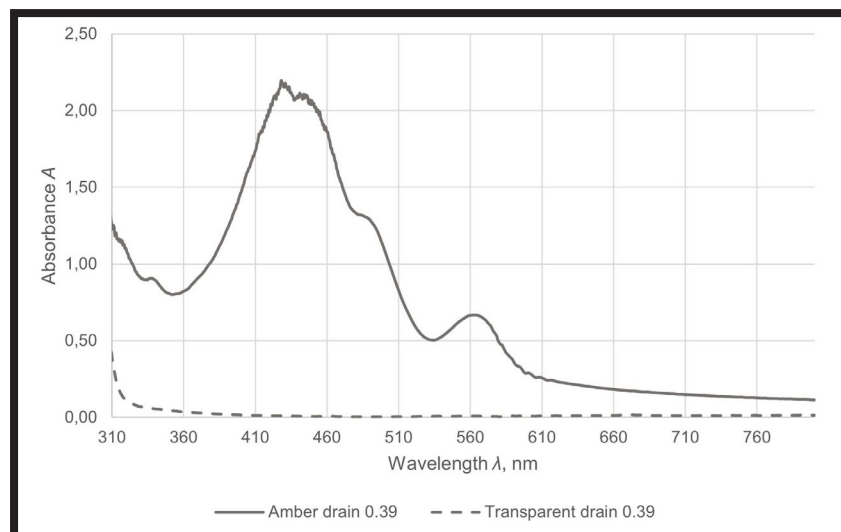
FIG. 13. Absorbance spectra of amber sample No. 4 and transparent sample No. 1.
