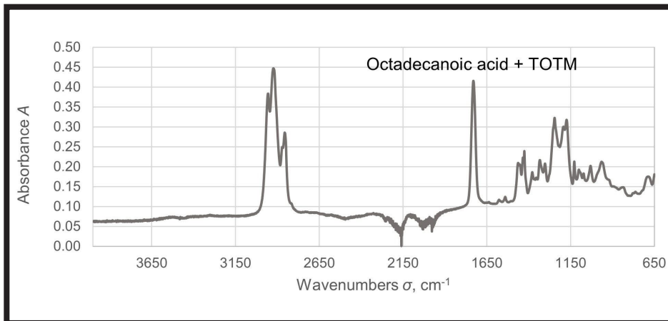
FIG. 10. FTIR-ATR absorption spectrum of the amber drain.
