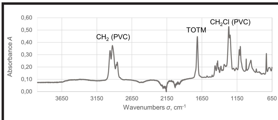
FIG. 11. FTIR-ATR absorption spectrum of the transparent drain.
