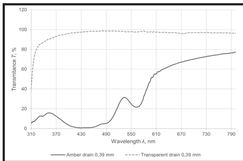
FIG. 12. Transmittance spectra of amber sample No. 4 and transparent sample No. 1.
