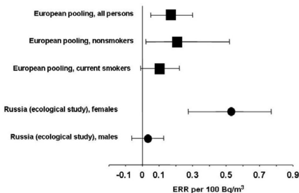
Fig. 6. Excess RR per 100 Bq/m 3 (European pooling – after correction for uncertainties [8]).
