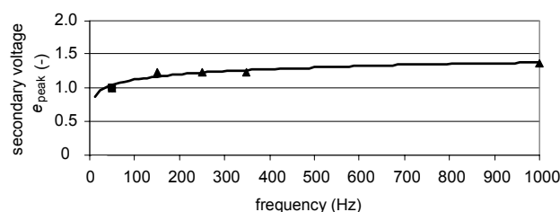
Fig. 5. Secondary voltage e_{\text{peak}} (peak value in relation to the reference value of 50 Hz) of the current transformer for the frequency range 50-1000 Hz for primary current I_{\Delta n} ; ( I_{\Delta n} is a rated residual current of the RCD)
