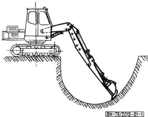
Fig. 1. Excavator equipped with backhoe equipment
