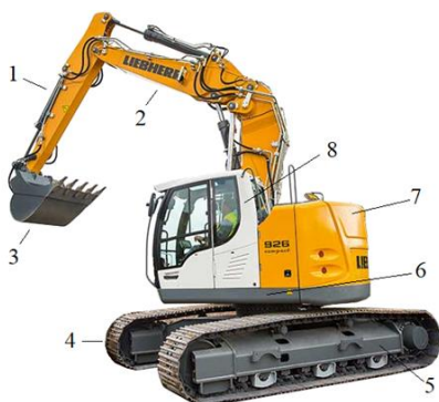
Fig. 3. Arrangement of the basic structural modules of a single-arm hydraulic backhoe on a crawler chassis
