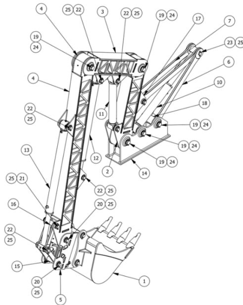
Fig. 12. Assembly drawing of finished attachments module
