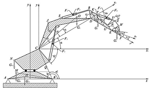
Fig. 2. Kinematic diagram of backhoe excavator with symbols
