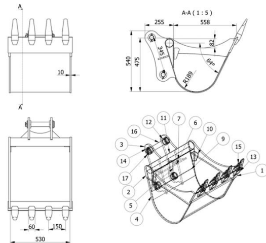
Fig. 9. Dimensions and assembly of designed bucket
