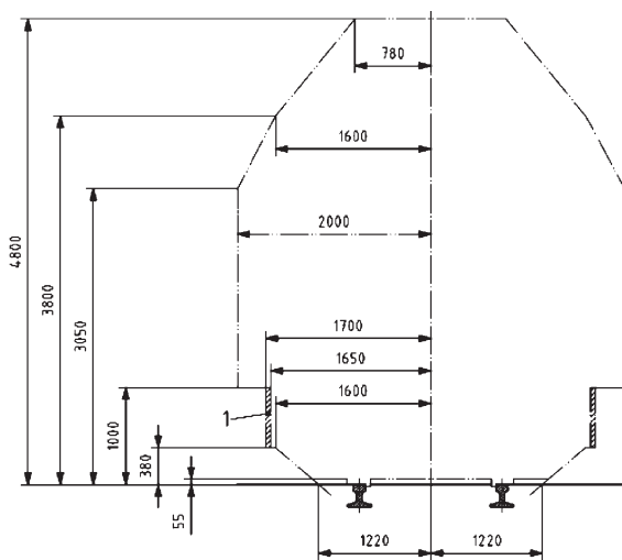
Fig. 3. Example of a structure gauge outline applied on European railways [8]: 1) platform edge mounting zone for platforms with heights from 550 to 1000 mm
