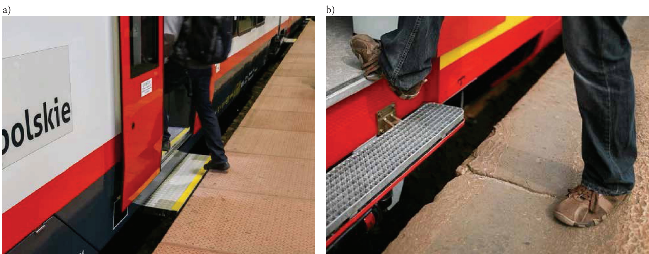
Fig. 20. Gap cover [39]: a) protractile, b) revolvable
