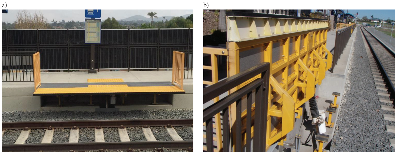
Fig. 12. View of a laid down footbridge (a) [4], laid up footbridge (b) [20]
