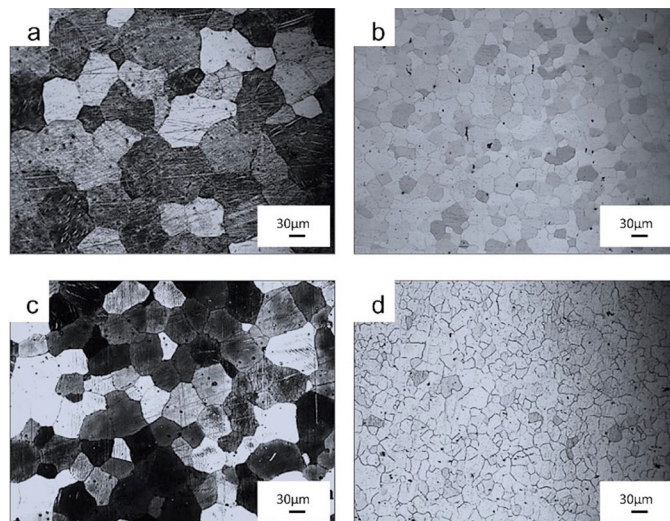
Fig. 2. Optical micrographs of the alloys: (a) as-cast ZM20, (b) as-rolled ZM20, (c) as-cast ZM21 and (d) as-rolled ZM21
