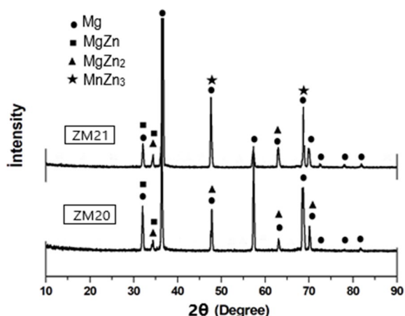
Fig. 1. XRD patterns of the alloys
