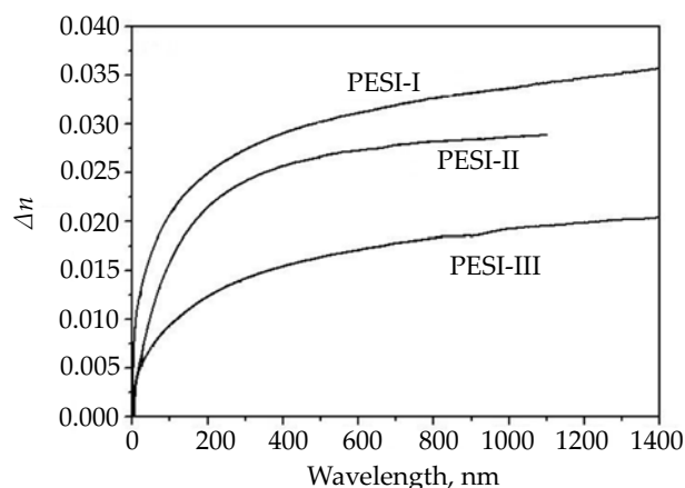
Fig. 1. The photoinduced birefringence of fully aromatic poly(ester imide)s
