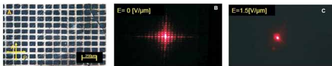
Fig. 3. A) Optical polarizing microscopy images of two-dimensional 2D gratings, visible diffraction patterns created from two-dimensional polarization gratings at: B) 0 V/μm, C) 1.5 V/μm applied electric field (1 kHz square wave)
