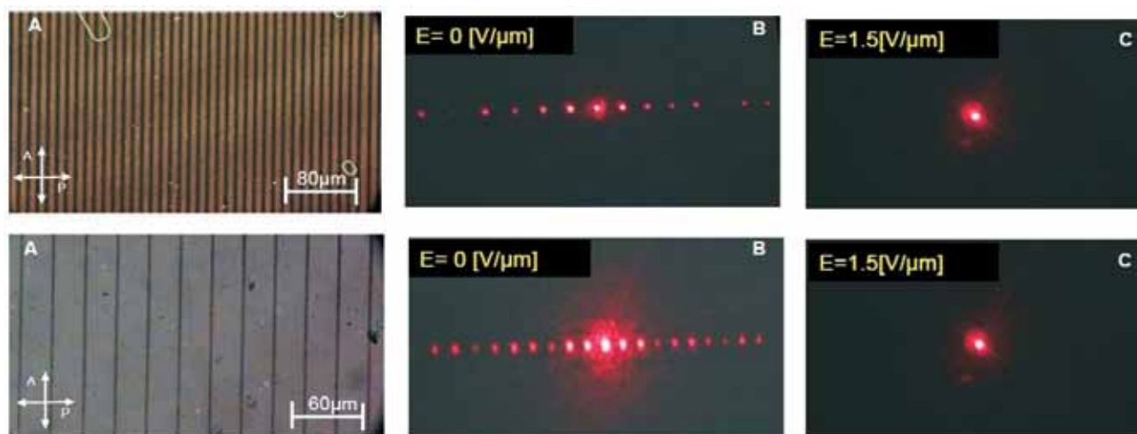
Fig. 2. A) Optical polarizing microscopy images of one-dimensional 1D gratings, visible diffraction patterns created from one-dimensional polarization gratings at: B) 0 V/μm, C) 1.5 V/μm applied electric field (1 kHz square wave)
