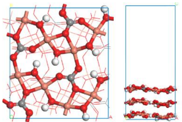
Fig. 14. Malachite (-201) surface
