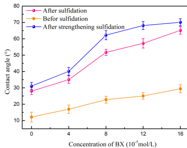
Fig. 7. Contact angles of malachite as function of BX dosages in the absence and presence of (NH 4 ) 2 SO 4 and Na 2 S
