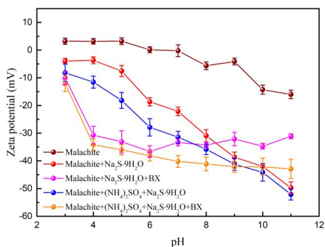
Fig. 8. Zeta potentials of malachite as function of pH in the absence and presence of (\text{NH}_4)_2\text{SO}_4 , \text{Na}_2\text{S} and NaBX
