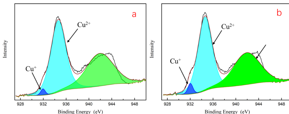
Fig. 13. Cu 2p spectra of malachite treated with (a) Na 2 S 9H 2 O and (b) (NH 4 ) 2 SO 4 + Na 2 S 9H 2 O
