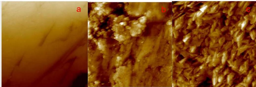
Fig. 11. AFM test of raw malachite(a) malachite treated with \text{Na}_2\text{S} \cdot 9\text{H}_2\text{O} (b), and malachite treated with (\text{NH}_4)_2\text{SO}_4 + \text{Na}_2\text{S} \cdot 9\text{H}_2\text{O} (c)
