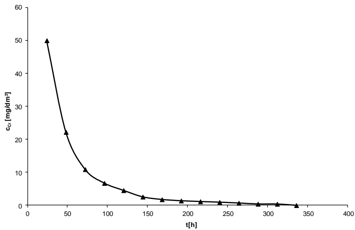
Figure 10. c_{Cr} = f(t) . Initial concentrations of chromium(VI) was 50 \text{ mg/dm}^3 ; \text{pH} = 4.5
