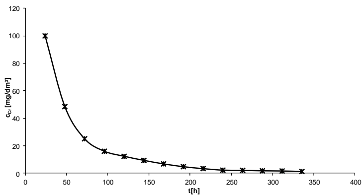
Figure 12. c_{Cr} = f(t) . Initial concentrations of chromium(VI) was 100 \text{ mg/dm}^3 ; \text{pH} = 4.5
