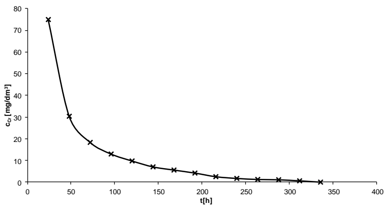
Figure 11. c_{Cr} = f(t) . Initial concentrations of chromium(VI) was 75 \text{ mg/dm}^3 ; \text{pH} = 4.5
