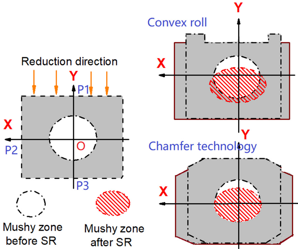
Fig. 16. Schematic of the deformation of the mushy zone at the bloom transverse section under different reduction cases
