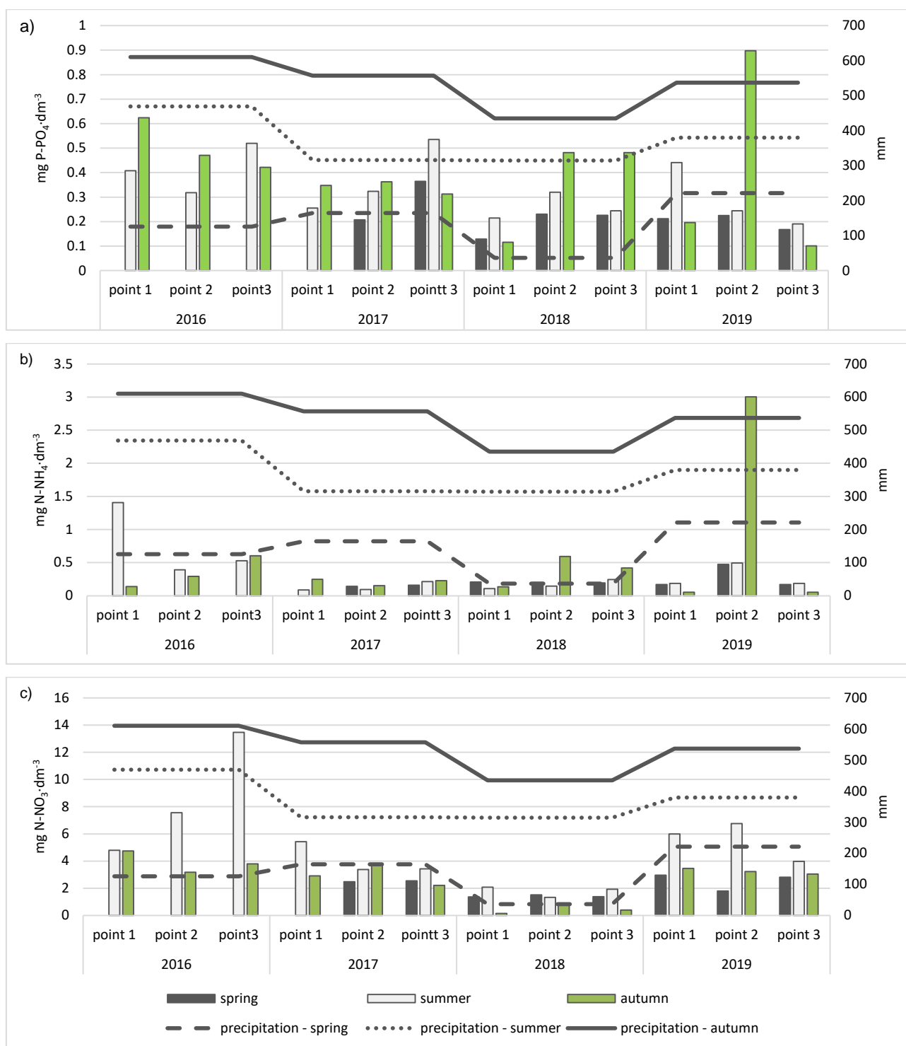
Fig. 3. The average concentration of fertilizer compounds vs. precipitation (spring, summer, autumn): a) \text{P-PO}_4 , b) \text{N-NH}_4 , c) \text{N-NO}_3 ; source: own study
