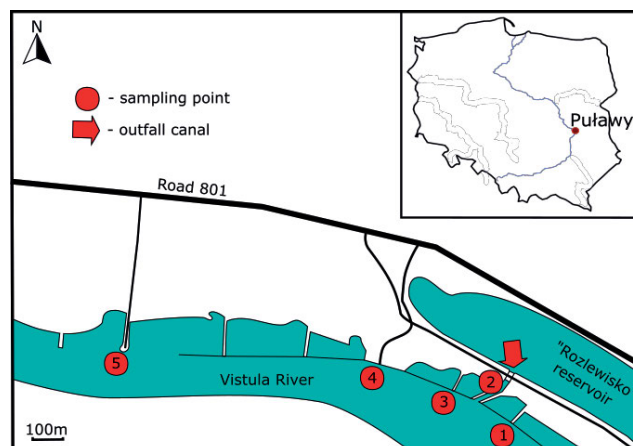
Fig. 1. Research area: location of outfall from "Rozlewisko" reservoir to the Vistula River and five sampling points. Location of Puławy city, Poland; source: own elaboration
