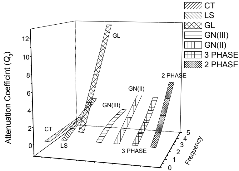
Fig.7. Variation of attenuation coefficient ( Q_3 ) with respect to frequency ( \omega ).
