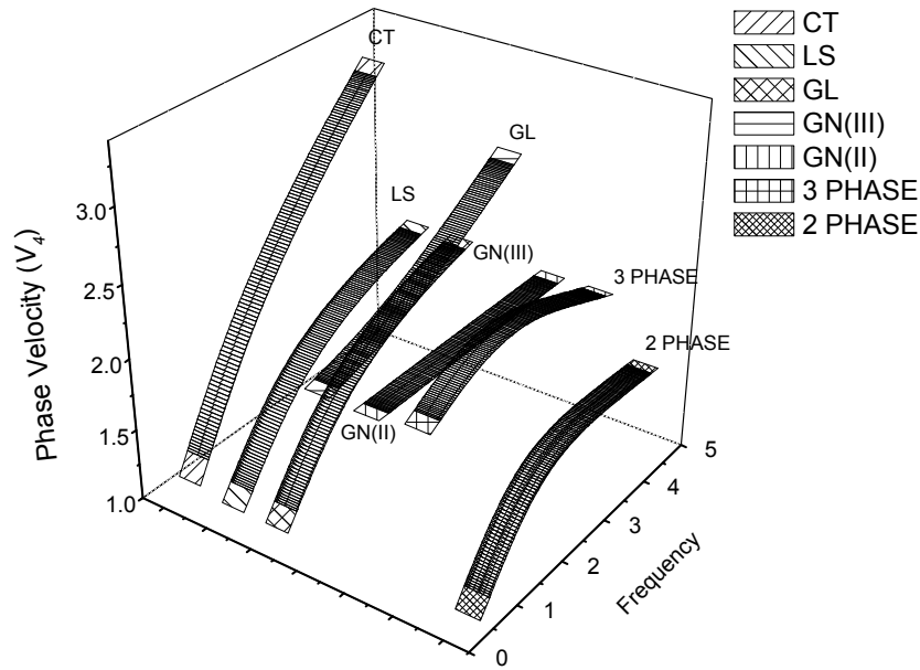
Fig.4a. Variation of phase velocity ( V_4 ) with respect to frequency ( \omega ).
