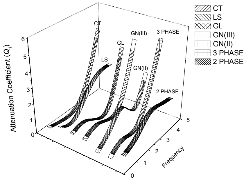
Fig.5. Variation of attenuation coefficient ( Q_1 ) with respect to frequency ( \omega ).
