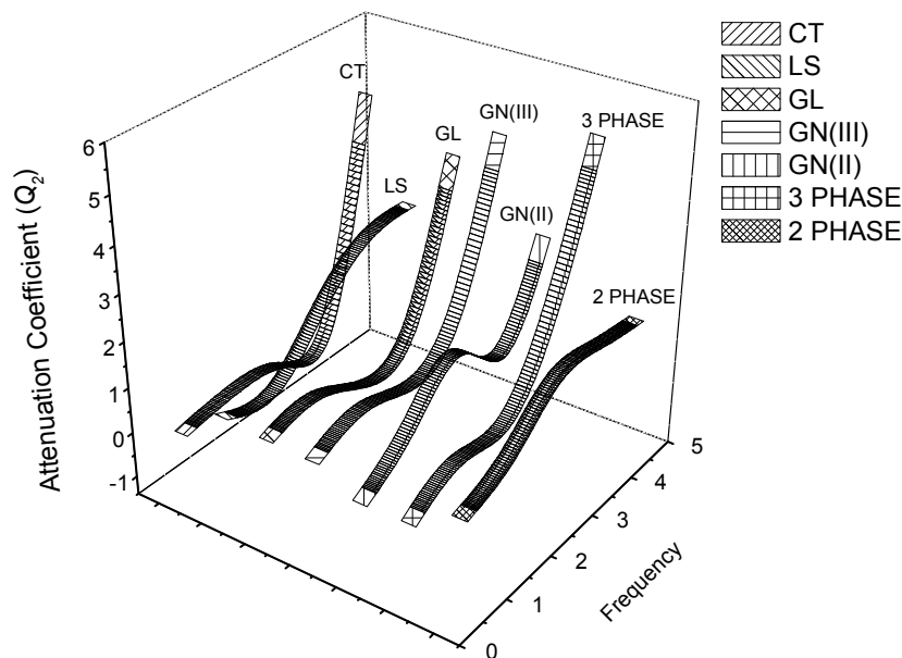
Fig.6. Variation of attenuation coefficient ( Q_2 ) with respect to frequency ( \omega ).
