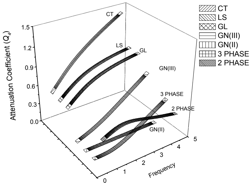
Fig.8. Variation of attenuation coefficient ( Q_4 ) with respect to frequency ( \omega ).
