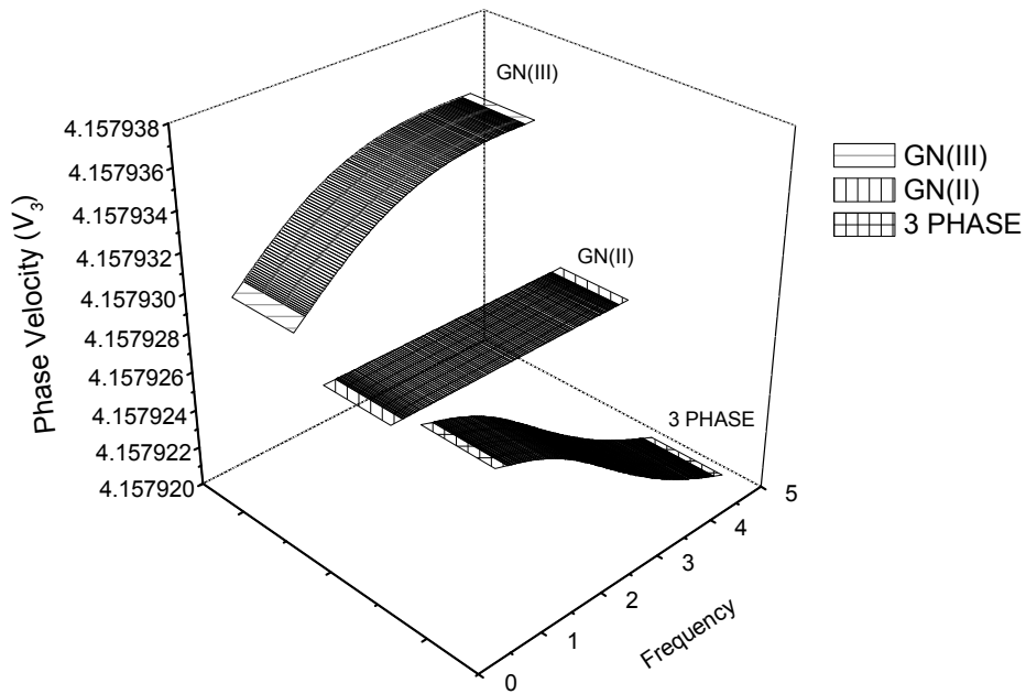
Fig.3b. Variation of phase velocity ( V_3 ) with respect to frequency ( \omega ).
