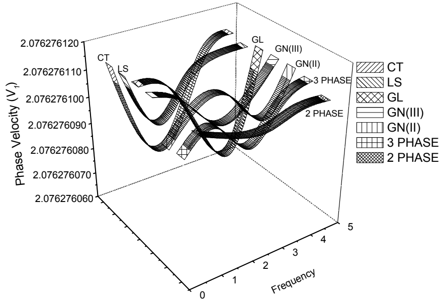
Fig.1. Variation of phase velocity ( V_1 ) with respect to frequency ( \omega ).
