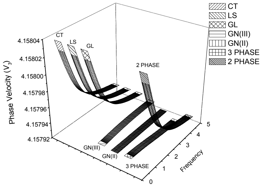
Fig.3a. Variation of phase velocity ( V_3 ) with respect to frequency ( \omega ).
