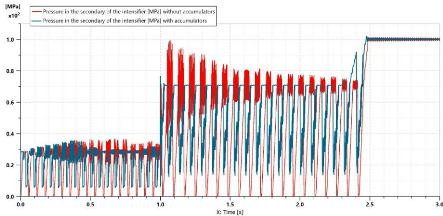
Fig. 7. Variation of the pressure in the secondary of the intensifier over time
