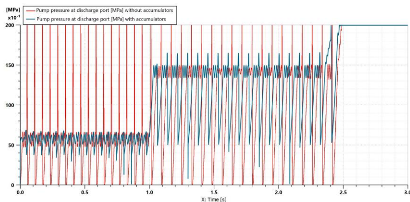
Fig. 3. Variation of the pressure at the discharge port of the hydraulic pump over time
