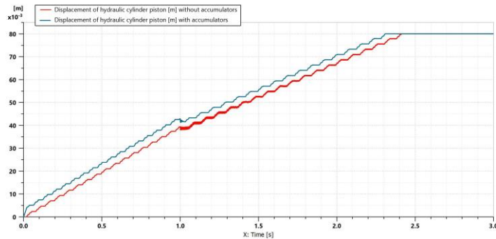
Fig. 11. Variation of the displacement of the hydraulic cylinder piston over time
