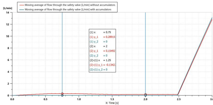
Fig. 4. Moving average of flow rate through the safety valve
