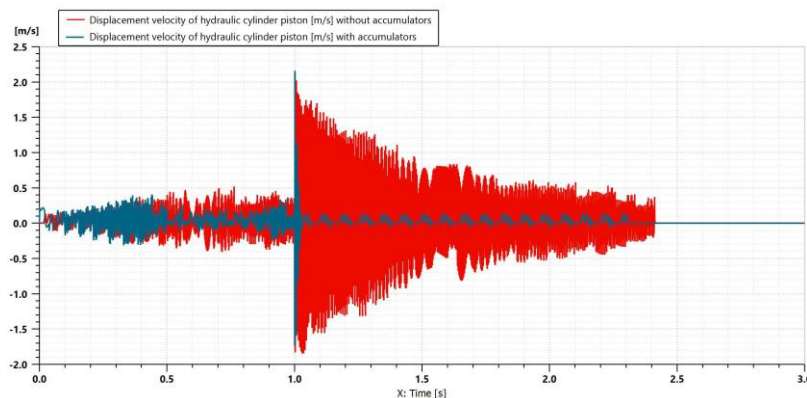
Fig. 13. Variation in time of the speed of movement of the hydraulic cylinder piston
