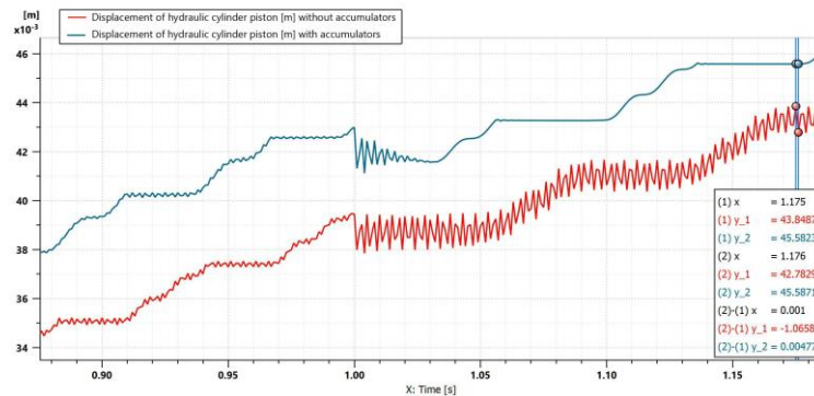
Fig. 12. Detail: displacement of the piston of the hydraulic cylinder
