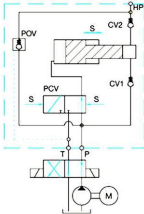
Fig. 1. Structure and operation of the SAOHPI: operating principle [11]
