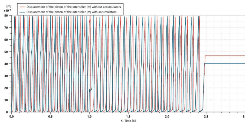
Fig. 5. Variation of the stroke of the hydraulic oscillator (intensifier's piston) over time
