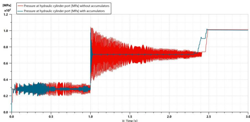
Fig. 8. Variation of the pressure at the port of hydraulic cylinder over time
