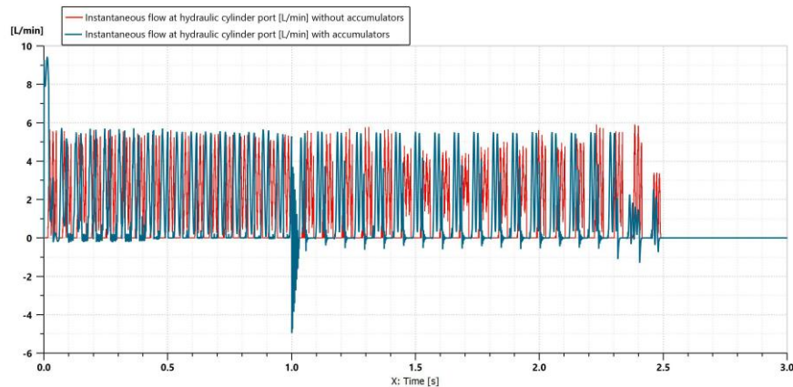
Fig. 9. Variation of the instantaneous flow rate at the hydraulic cylinder port over time
