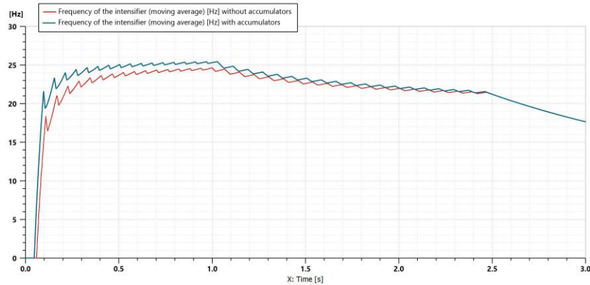
Fig. 6. Variation of the moving average frequency of the hydraulic oscillator (intensifier piston) over time
