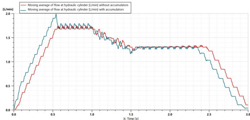
Fig. 10. Variation of the moving flow rate average at the hydraulic cylinder port over time
