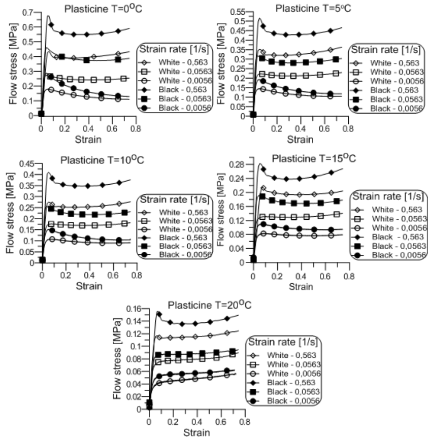
Fig. 1. Plasticine flow curves at temperatures of 0, 5, 10, 15, 20 °C
