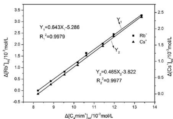
Figure 8. The change of concentrations of Rb + , Cs + and C 4 mim + in the aqueous phase before and after the extraction in the 18C6/[C 4 mim][PF 6 ] system
