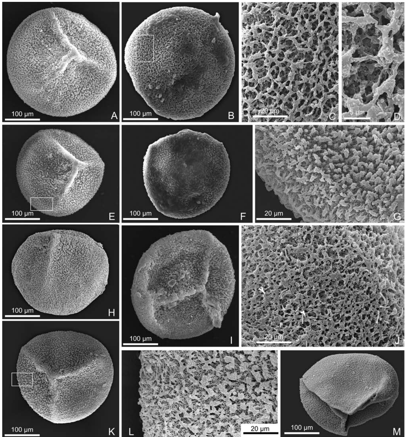
Fig. 5. Induan megaspores from Sholga locality. A–M – Maexisporites rugulaeferus sp. nov.; A–D – holotype, specimen PIN 5529/113: A–B – proximal and distal view, C, D – details of distal wall showing sculpture; E–G – specimen PIN 5529/105: E, F – proximal and distal view, G – detail of proximal wall showing sculpture; H – specimen PIN 5529/47, oblique compression, note finer sculpture over the distal hemisphere; I, J – specimen PIN 5529/100: I – proximal view, J – detail of proximal wall showing sculpture; K, L – specimen PIN 5529/43: K – proximal view, L – detail of proximal wall showing sculpture; M – specimen PIN 5529/46, oblique compression.
