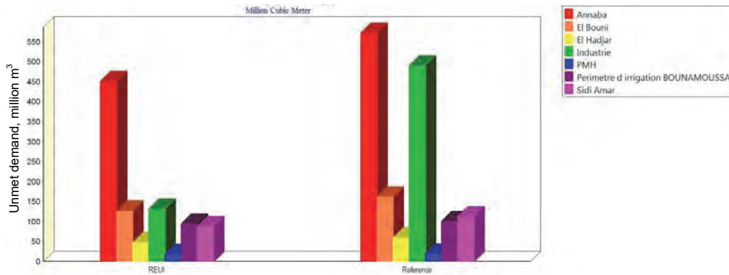
Fig. 8. Comparison of unmet demand of both scenarios Reference and Industrial Water Reuse (REUI); source: own study
