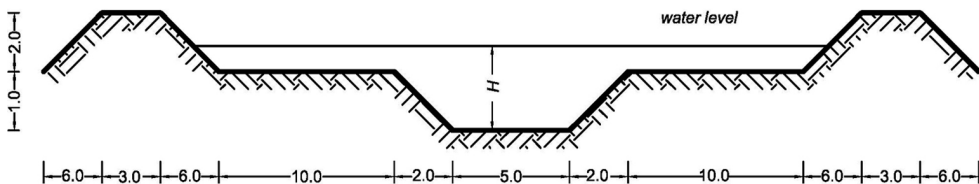
Fig. 1. The cross-section of the designed river channel. The scale of the image has not been kept
