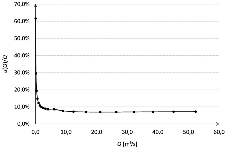
Fig. 3. A graph of the percentage dependence of the u(Q)/Q ratio of the uncertainty of discharge to the calculated value of the discharge
