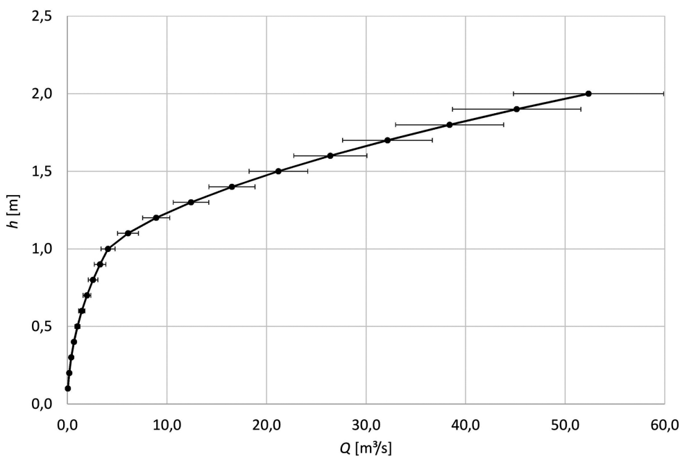
Fig. 2. The rating curve with marked intervals of expanded uncertainty
