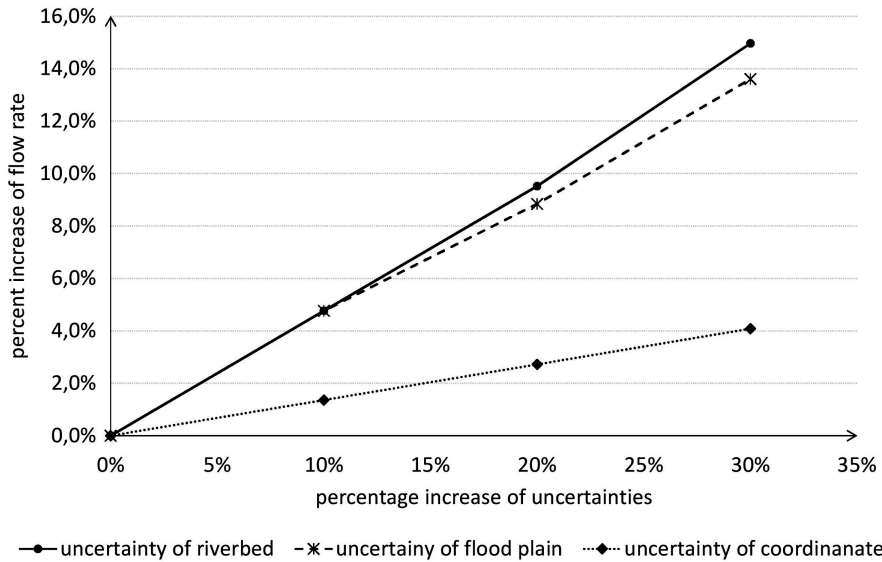
Fig. 4. The dependence of the influence of the percentage change of the uncertainty of roughness coefficients of the channel, of the floodplain, and of the uncertainty of the geometric dimensions of the river channel water area on the uncertainty of the discharge
