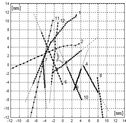
Fig. 8. Safe trajectory of the own ship for the PG_c algorithm in restricted visibility D_s = 2 nm in a situation of passing j = 12 encountered ships, r(t_k) = 0 , d(t_k) = 1.40 nm.
