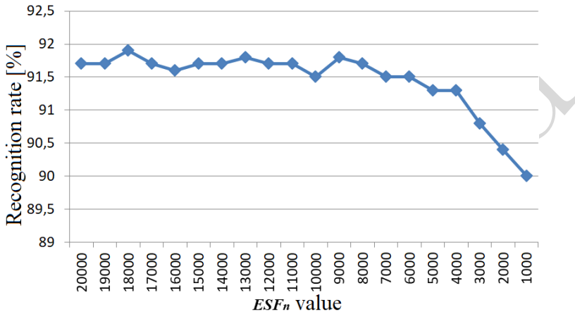
Figure 9. Recognition rates (in [%] on vertical axis) obtained using DS_R dataset depending on ESF_n parameter value (horizontal axis)
