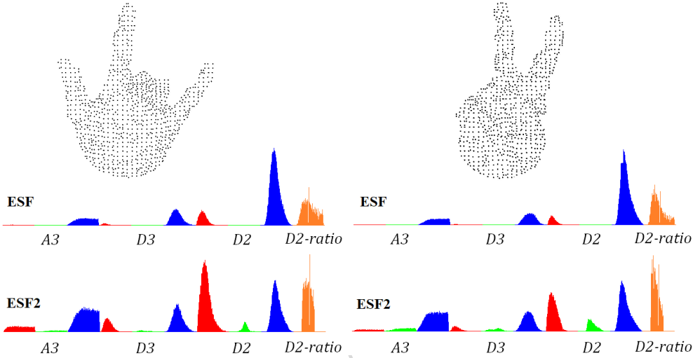
Figure 3. ESF histograms generated for all point clouds representing two hand postures: sub-histograms IN and MOSTLY-IN marked in red; OUT and MOSTLY-OUT - green; MIXED - blue; D2 - ratio histogram marked in orange
