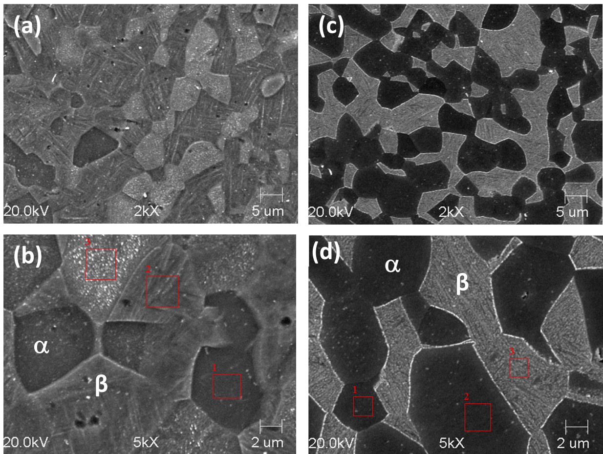
Fig. 2. Microstructure of Ti-6Al-4V specimens revealed after chemical etching in the Kroll's solution. Figures (a,b) for the Ti-6Al-4V_HT_950 and (c,d) for the Ti-6Al-4V_HT_950 + 500, respectively
