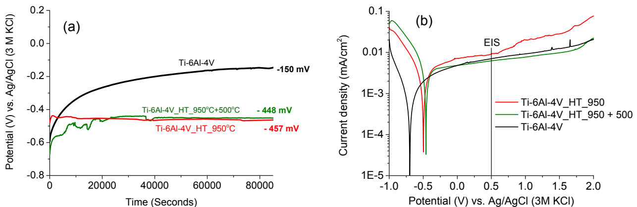
Fig. 4. The evolution of open circuit potential (a) and potentiodynamic polarization curves (b) obtained for Ti-6Al-4V and Ti-6Al-4V_HT specimens in artificial saliva at 37^{\circ}\text{C}
