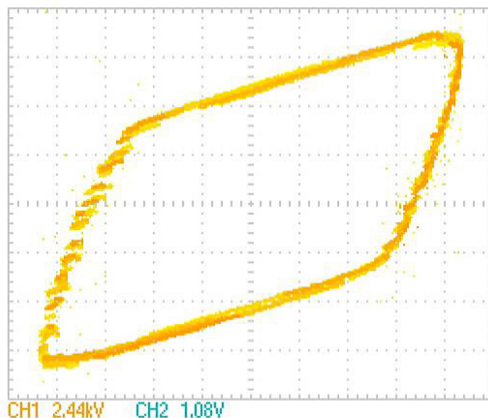
Fig. 5. Figure Lissajous figures for micanite dielectric for discharge gap 2.0 mm, electrodes with holes \text{Ø}1.38 mm, at supply voltage V = 10200V .
