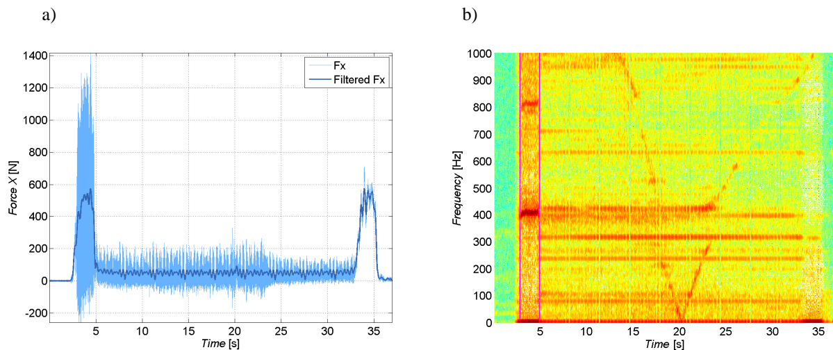
Fig. 10. Cutting force signal ( F_x ) and corresponding spectrogram indicating chatter on a 40×40 mm hollow profile: a) Force signal on a 40×40 mm square hollow profile, b) Force spectrogram shows some emphasized frequencies
