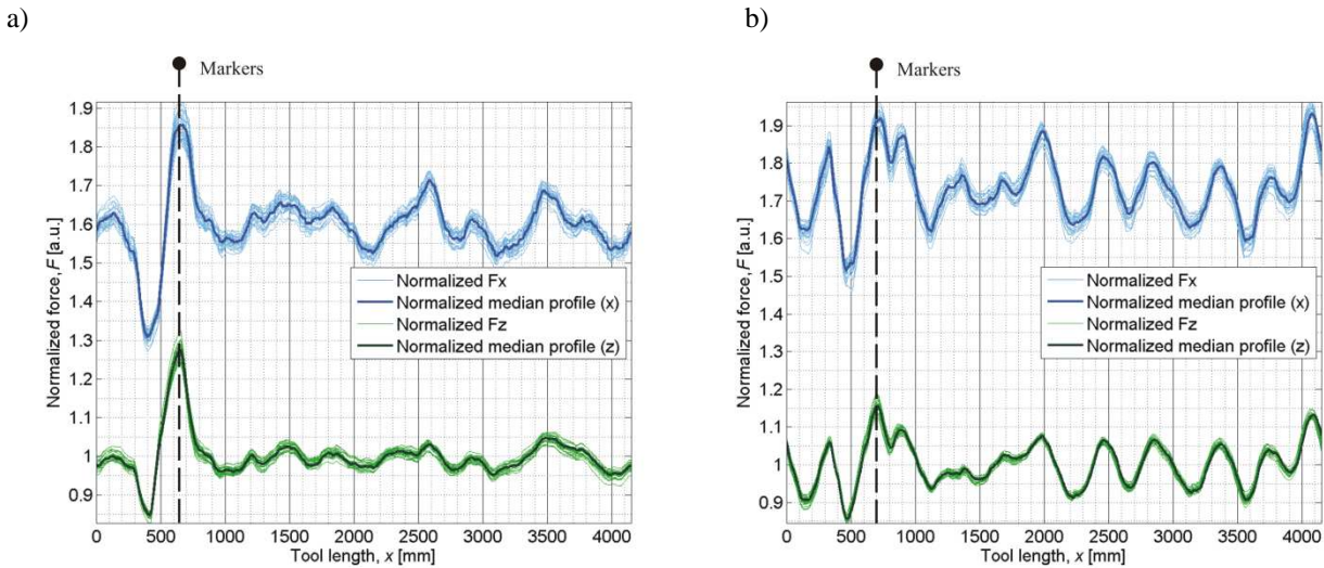
Fig. 9. Comparison of two different blades' force profiles obtained at the same cutting parameters: a) normalized geometry of blade 1, b) normalized geometry of blade 2
