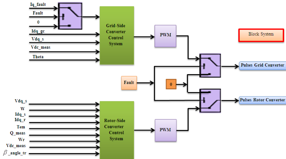
Fig. 8. Diagram of blocking converters
