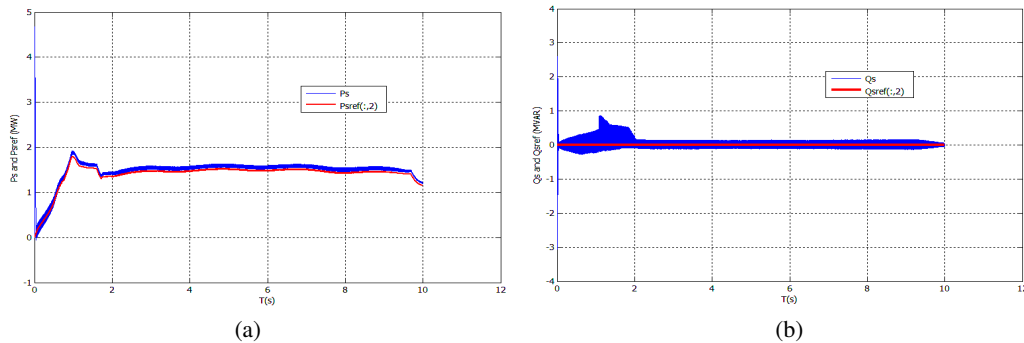
Fig. 15. (a) measured active power and reference power, (b) measured reactive power and reference power
