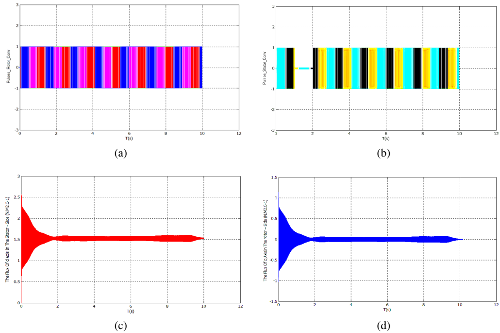
Fig. 12. (a) rotor-side converter pulses, (b) stator-side converter pulses, (c) the flux of d -axis the stator-side, (d) the flux of q -axis the rotor-side
